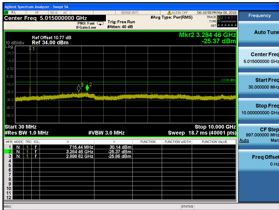
LTE Band 12 / 1.4MHz / QPSK - RB Size/Offset (6/0) – High Channel
