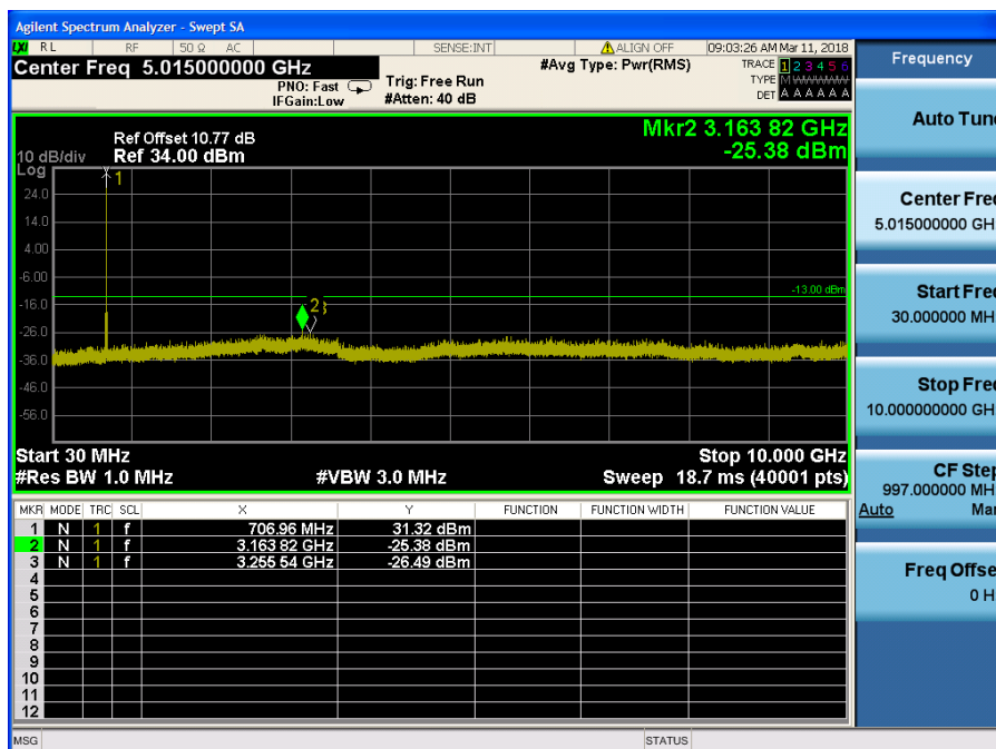
LTE Band 17 / 10MHz / 64QAM - RB Size/Offset (1/0) – High Channel
