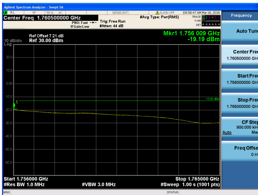
LTE Band 4 / 10MHz / QPSK - RB Size/Offset (50/0)
