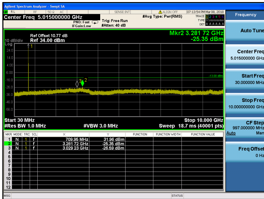
LTE Band 12 / 5MHz / QPSK - RB Size/Offset (1/24) – Mid Channel
