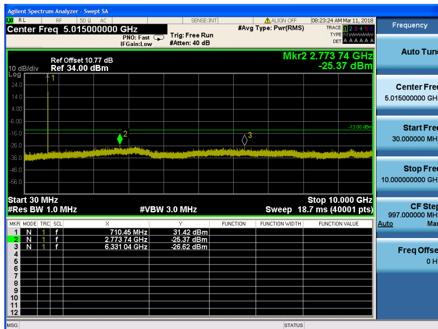
LTE Band 17 / 5MHz / 64QAM - RB Size/Offset (1/12)–Mid Channel
