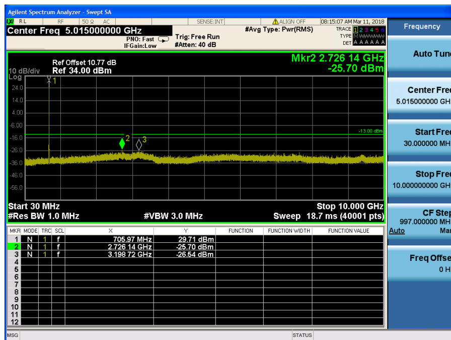
LTE Band 17 / 5MHz / 64QAM - RB Size/Offset (12/0) – Low Channel
