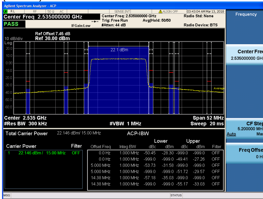
LTE Band 7 / 15MHz / 64QAM - RB Size/Offset (75/0)
