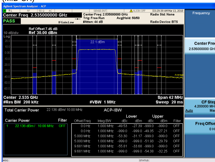
LTE Band 7 / 10MHz / 64QAM - RB Size/Offset (50/0)
