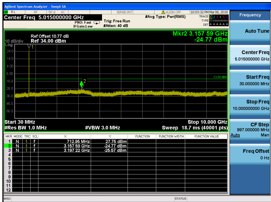
LTE Band 12 / 5MHz / 16QAM - RB Size/Offset (25/0) – High Channel
