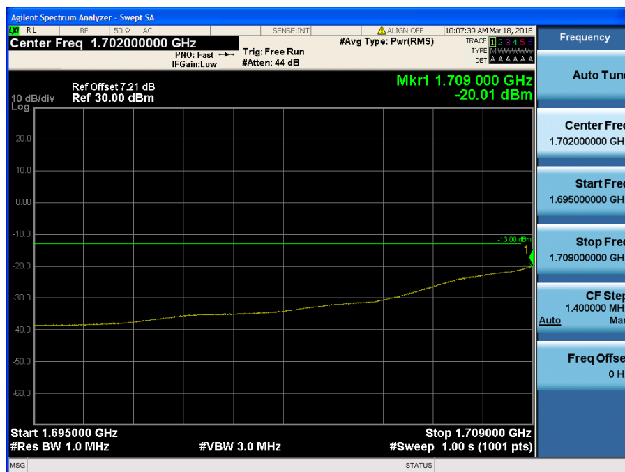
LTE Band 4 / 15MHz / QPSK - RB Size/Offset (36/0)
