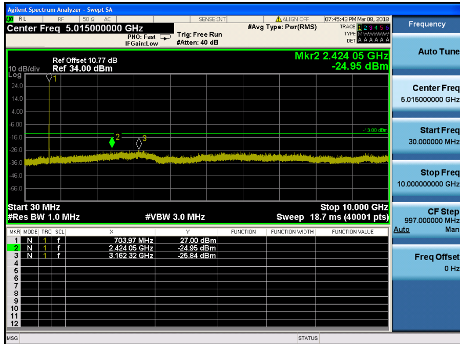
LTE Band 12 / 10MHz / QPSK - RB Size/Offset (25/12) – Low Channel
