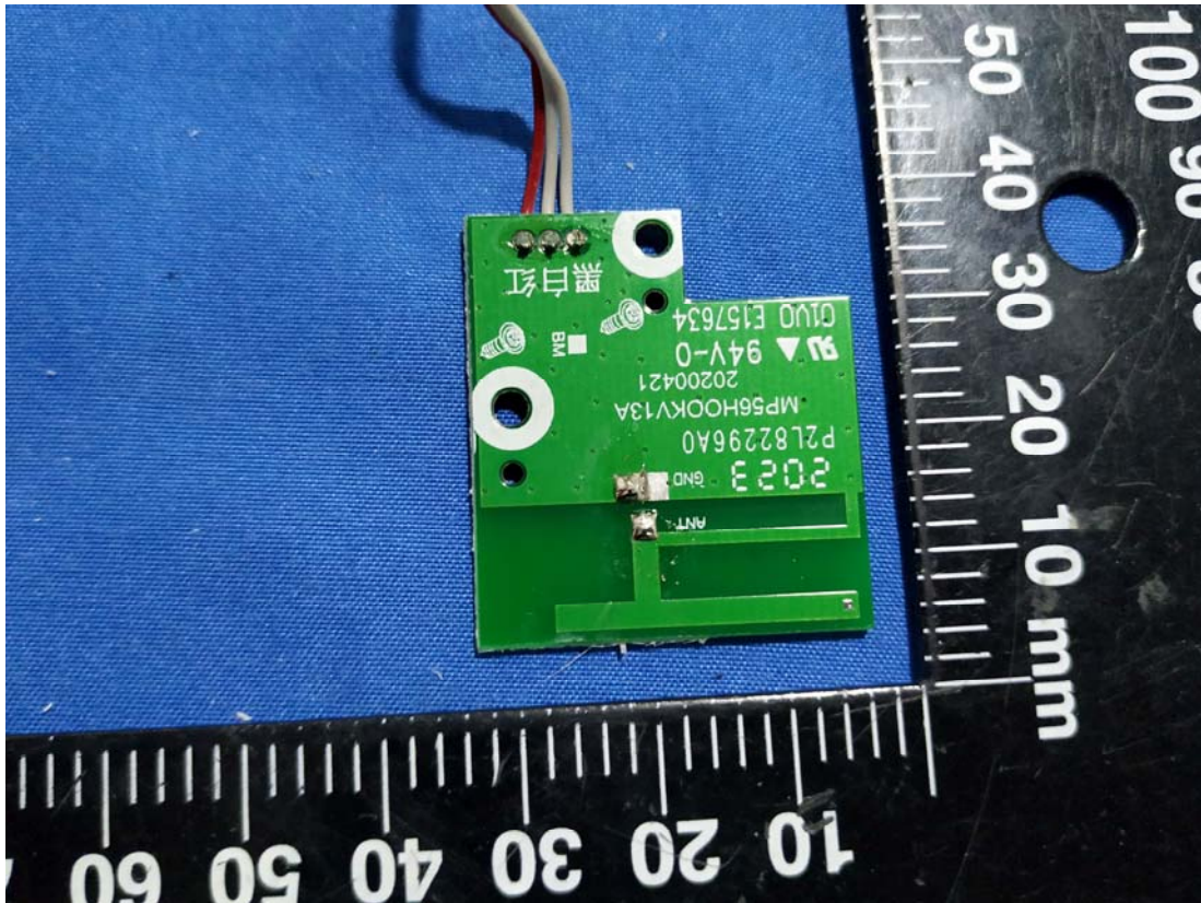
WiFi/BT Antenna
