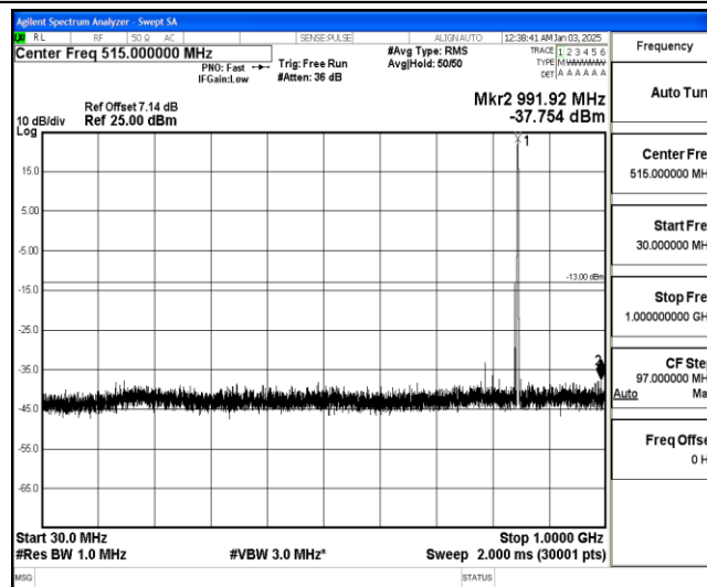
Band26-1.4MHz-QPSK-27033-1-0-High-30-1000--37.75-PASS
