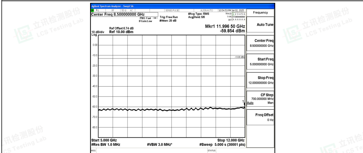
Band26-1.4MHz-QPSK-26697-1-0-Low-5000-12000--59.85-PASS
