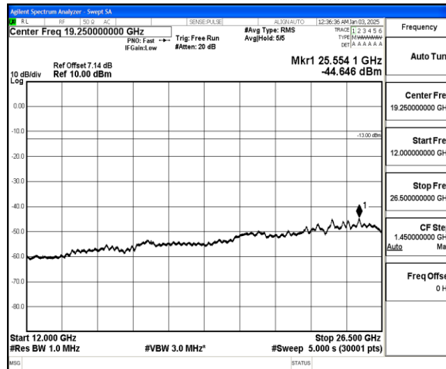
Band26-1.4MHz-QPSK-26915-1-0-Low-12000-26500--44.65-PASS
