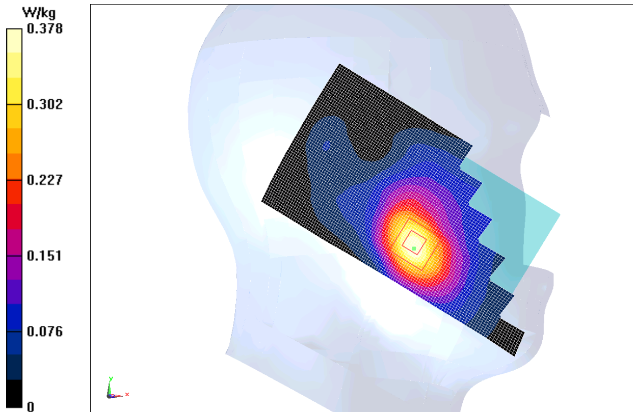
Fig.3 1900 MHz CH810
