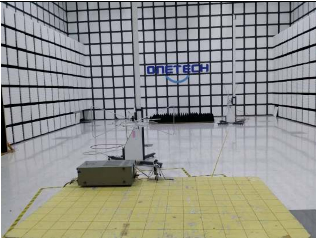
Installed 'Z' orientation
