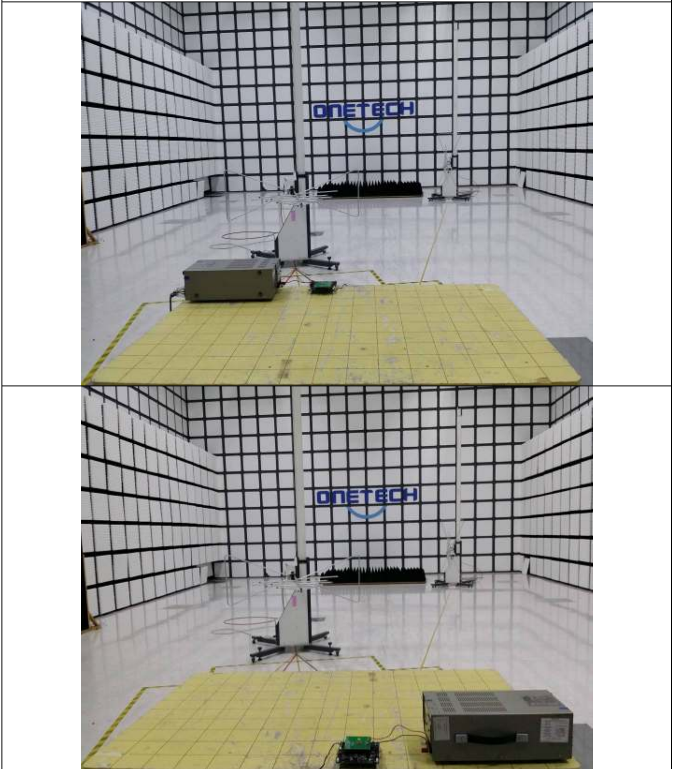
Installed 'X' orientation
