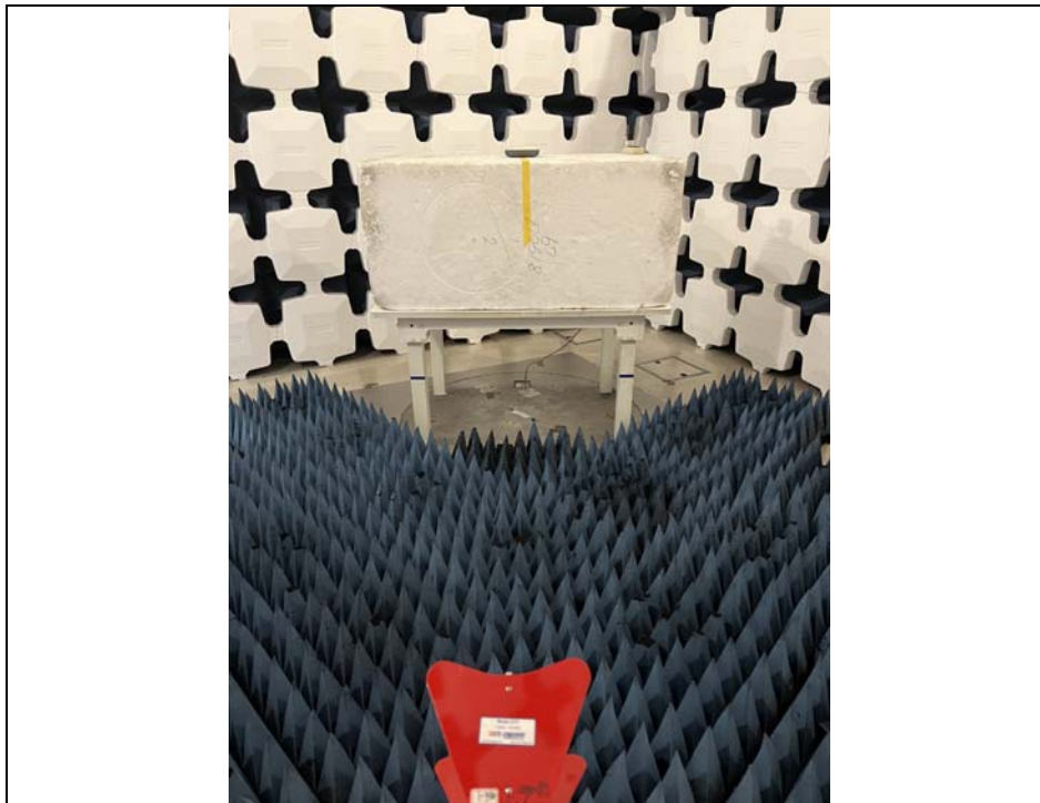
Radiated Emission Test (Above 1GHz) (Adapter Mode: X plane)
