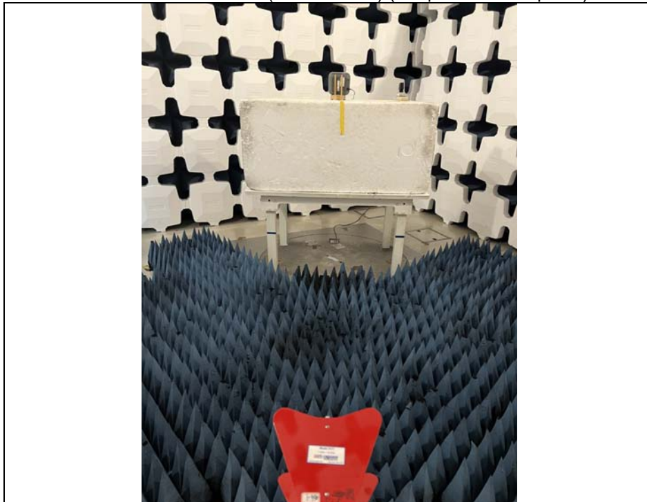
Radiated Emission Test (Above 1GHz) (Adapter Mode: Y plane)
