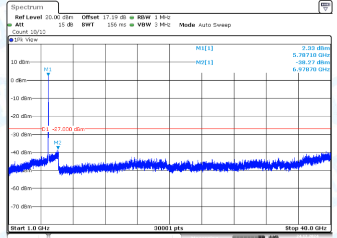
11N40SISO-Ant1-5795-1000~40000-PASS
