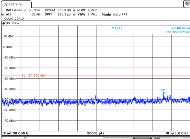
11N40SISO-Ant1-5795-30~1000-PASS
