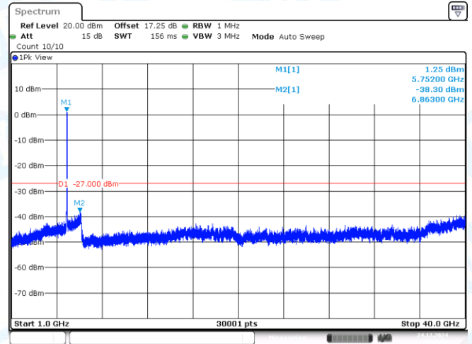
11AC40SISO-Ant1-5755-1000~40000-PASS
