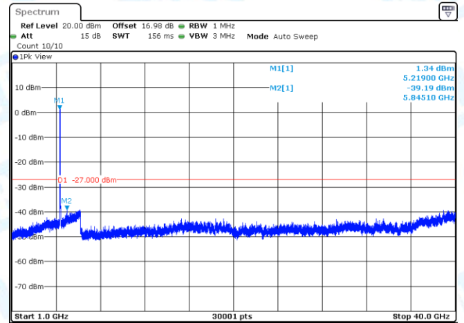
11AC40SISO-Ant1-5190-1000~40000-PASS
