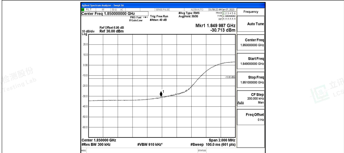
Band2-15MHz-QPSK-19125-75RB#0
