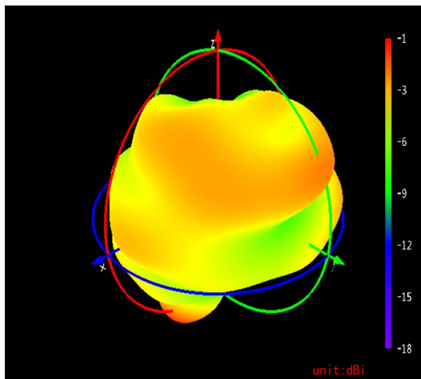
Radiation pattern @2.480GHz
