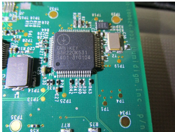
RF MAIN CHIP
