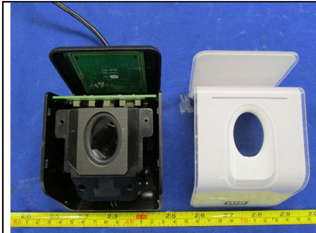
Cover off View 1
