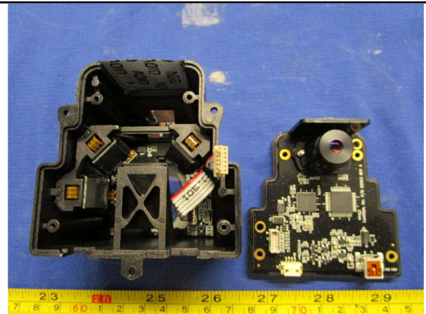
Cover off View 2 with PCBA1
