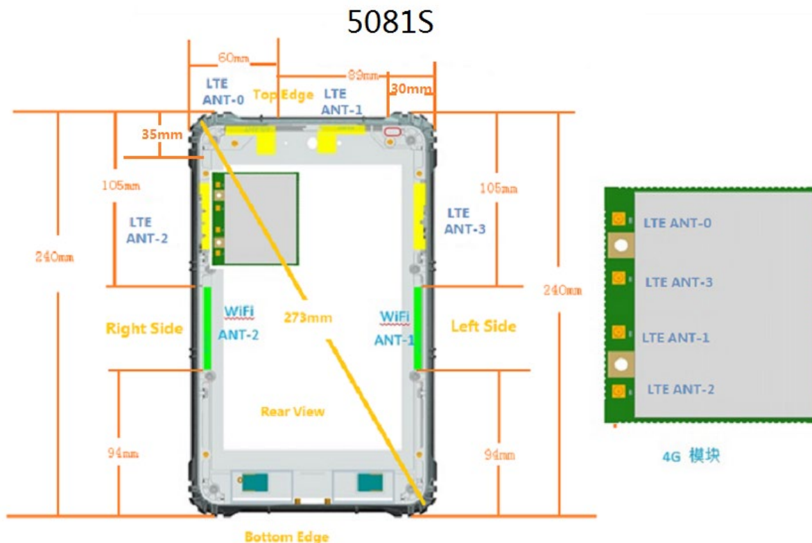
Figure: The location of the antennas
