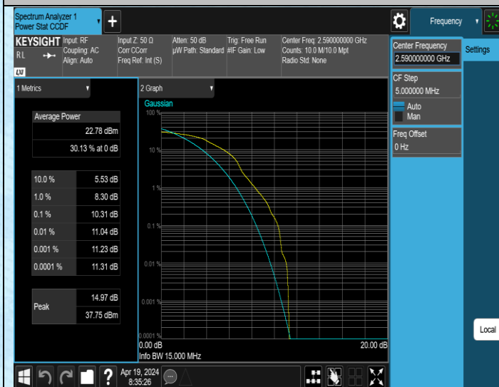
41(2535-2655)-15MHz-16QAM-40590-1RB#0-PASS
