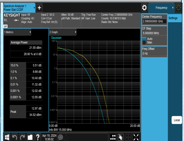
41(2535-2655)-15MHz-16QAM-40590-75RB#0-PASS
