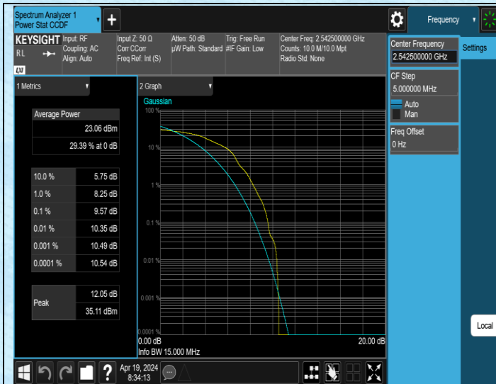
41(2535-2655)-15MHz-16QAM-40115-1RB#0-PASS
