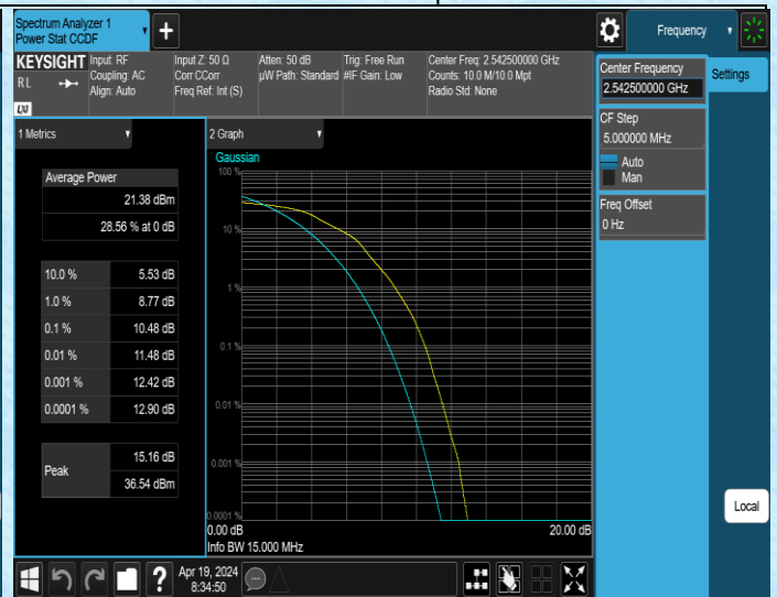
41(2535-2655)-15MHz-16QAM-40115-75RB#0-PASS
