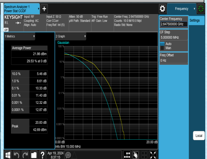
41(2535-2655)-15MHz-16QAM-41165-75RB#0-PASS
