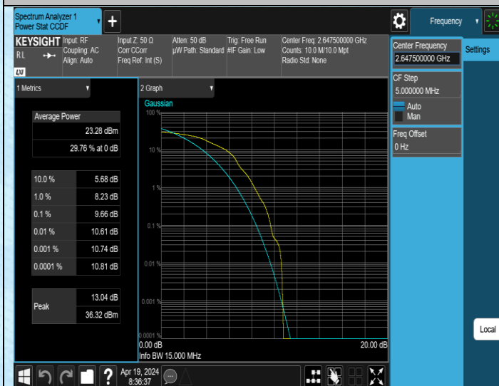
41(2535-2655)-15MHz-16QAM-41165-1RB#0-PASS
