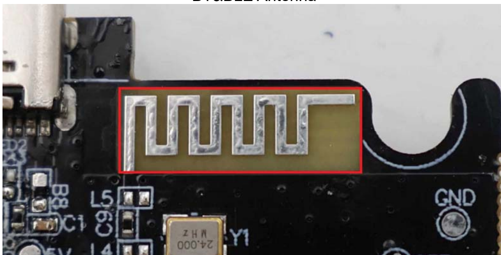
BT&amp;BLE Antenna
