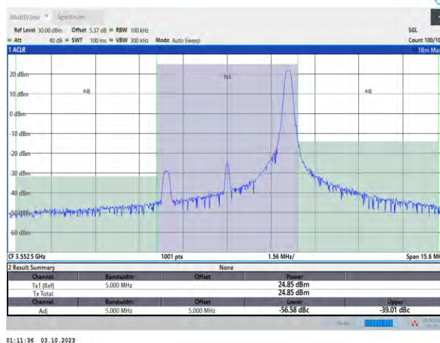
Band48-5MHz-QPSK-55265-1RB#24
