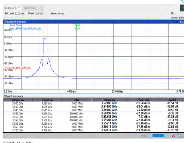
Band48-5MHz-QPSK-55265-25RB#0
