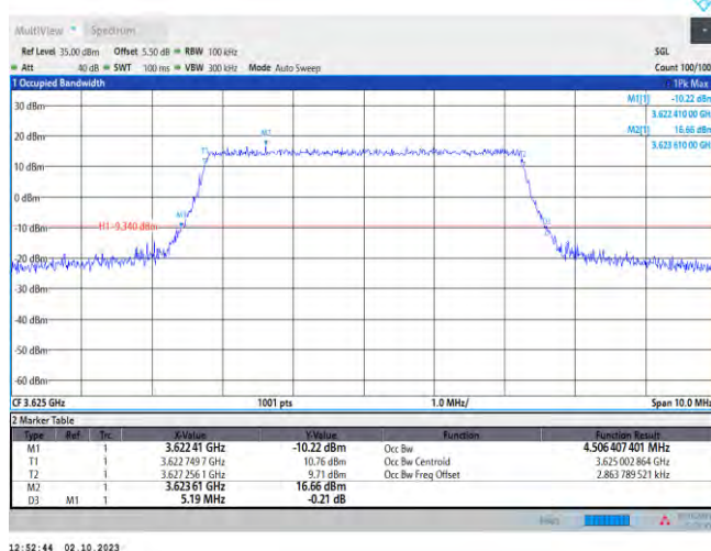
Band48-5MHz-16QAM-55990-25RB#0
