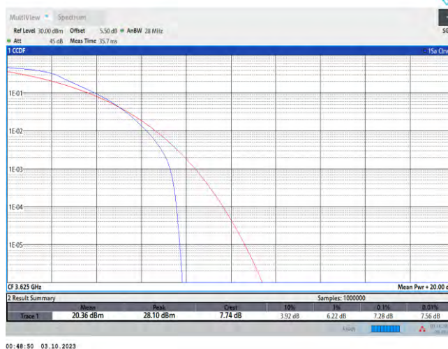
Band48-20MHz-QPSK-55990-100RB#0
