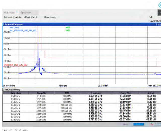
Band48-5MHz-QPSK-55265-25RB#0
