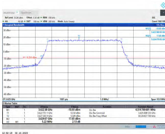
Band48-5MHz-16QAM-55990-25RB#0
