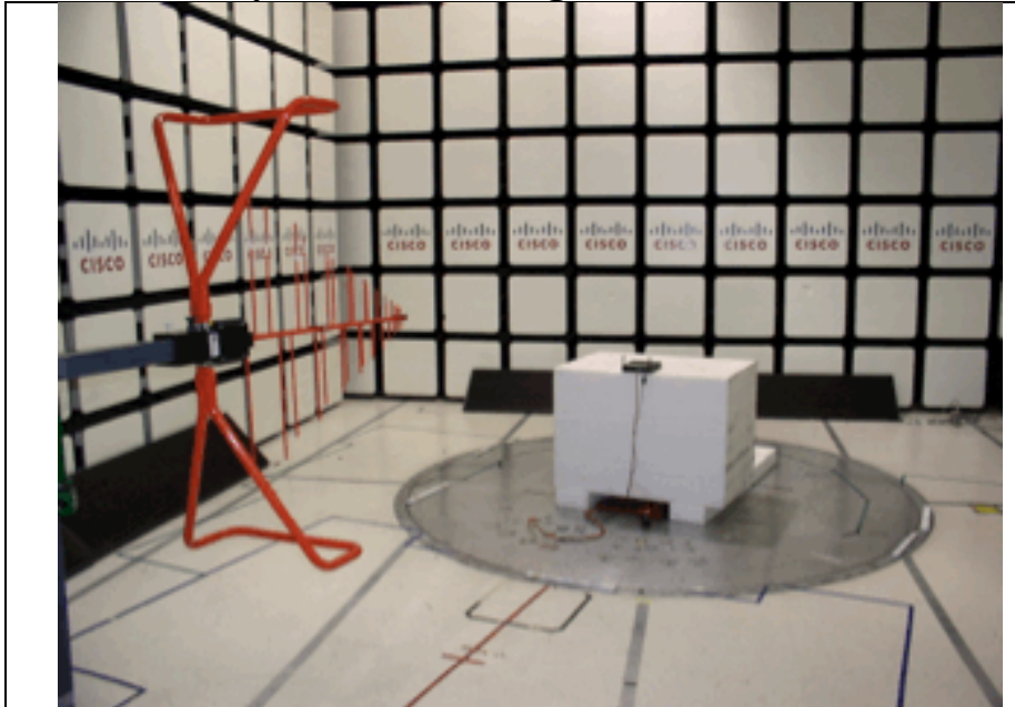
Title: Radiated Emissions Below 1 GHz
