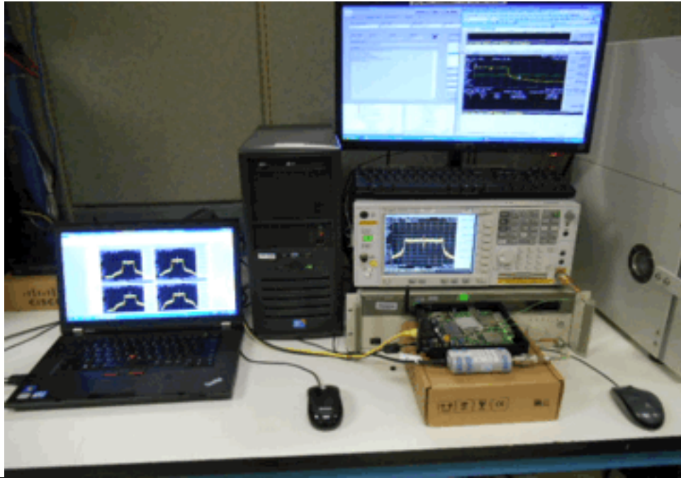
Title: RF Conducted Test Setup
