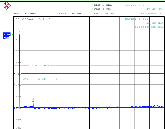
Test Mode: LTE Band 66 / 1.4MHz /1RB
