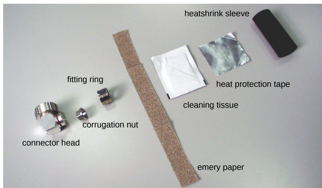
Fig. 2.45 Parts of the connector unit kit (example)
