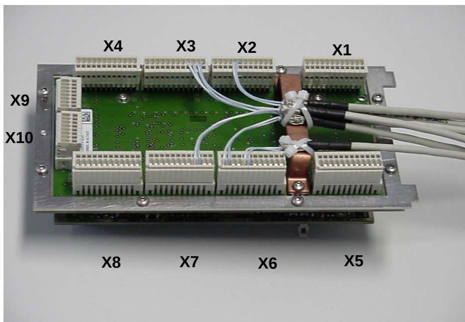
Fig. 2.41 ACTM terminal numbering
