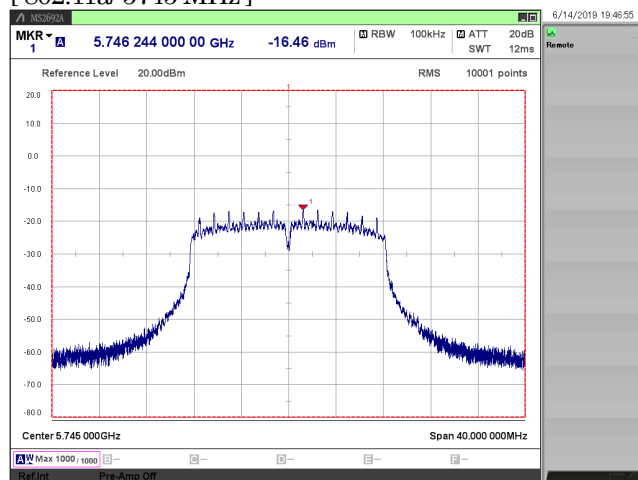
[ 802.11a/ 5745 MHz ]
