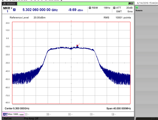
[ 802.11a/ 5300 MHz ]
