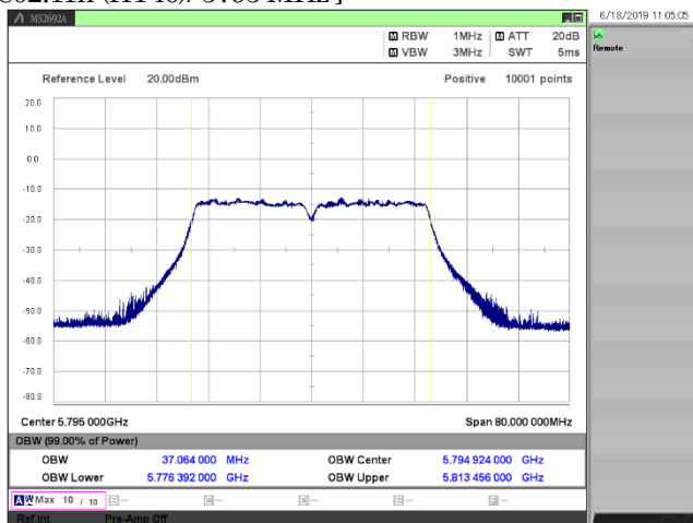
[ 802.11n (HT40)/ 5795 MHz ]
