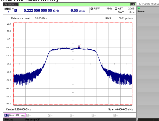
[ 802.11a/ 5220 MHz ]
