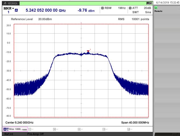
[ 802.11a/ 5240 MHz ]
