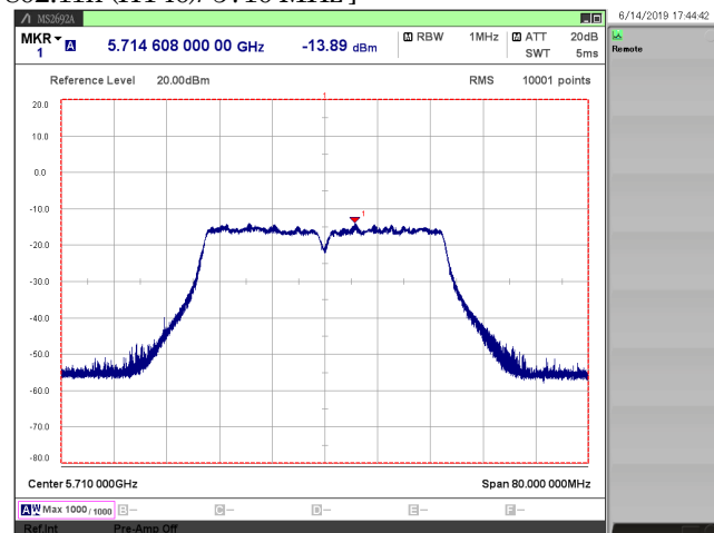
[ 802.11n (HT40)/ 5710 MHz ]
