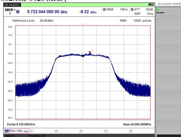
[ 802.11a/ 5720 MHz ]
