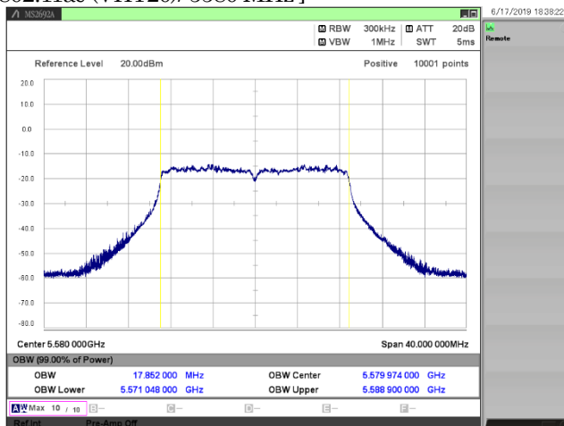
[ 802.11ac (VHT20)/ 5580 MHz ]
