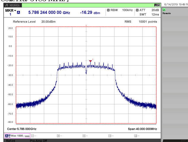
[ 802.11a/ 5785 MHz ]
