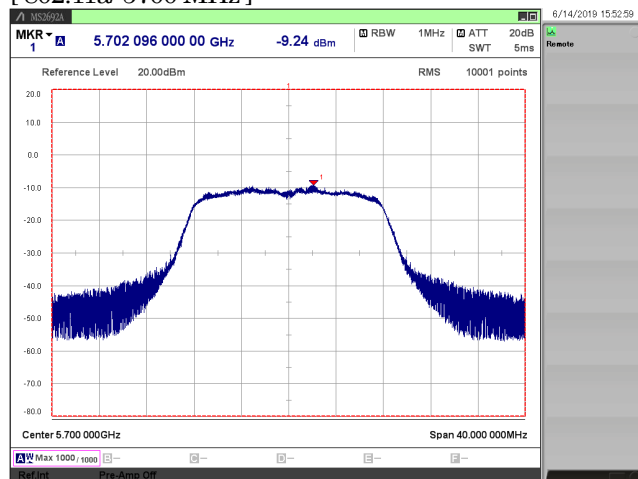
[ 802.11a/ 5700 MHz ]
