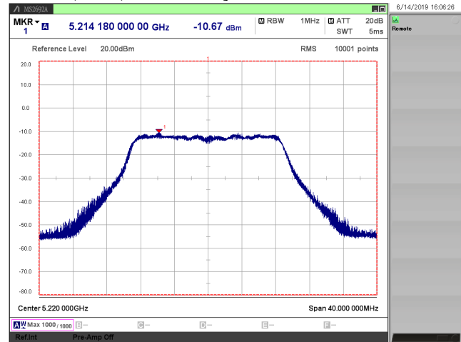
[ 802.11n (HT20)/ 5220 MHz ]
