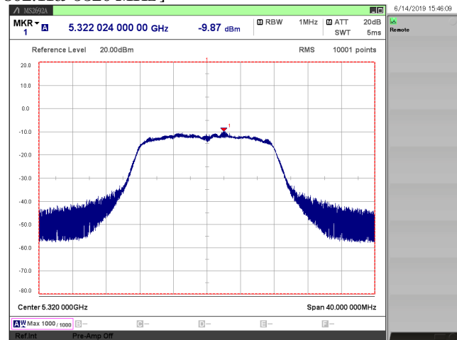
[ 802.11a/ 5320 MHz ]
