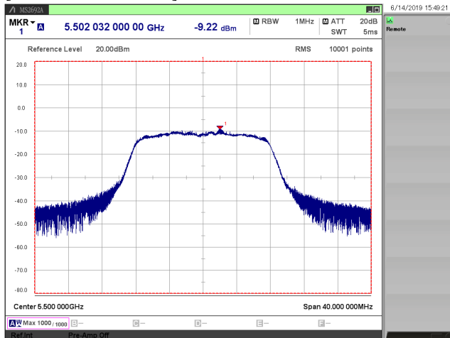
[ 802.11a/ 5500 MHz ]
