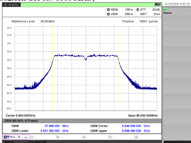
[ 802.11n (HT40)/ 5550 MHz ]
