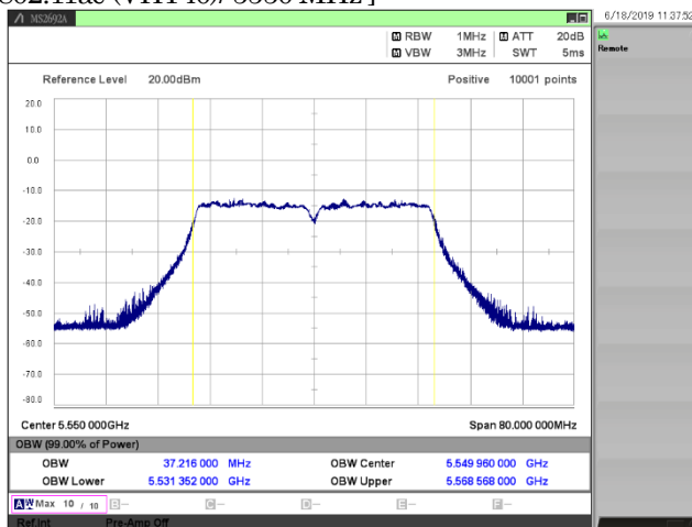
[ 802.11ac (VHT40)/ 5550 MHz ]
