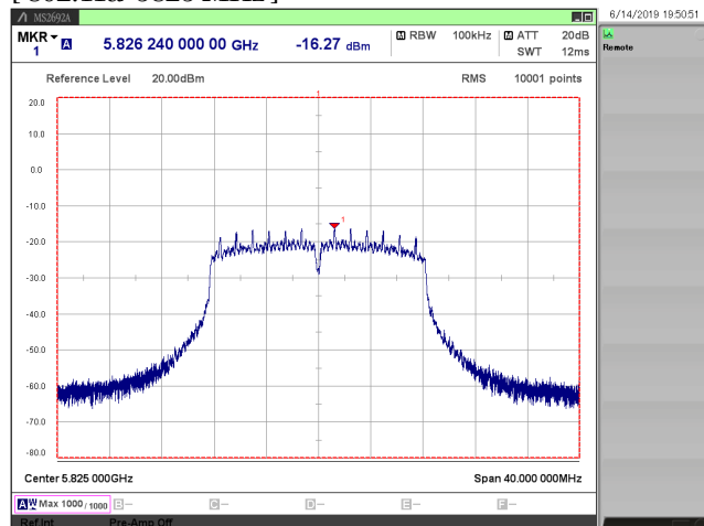
[ 802.11a/ 5825 MHz ]
