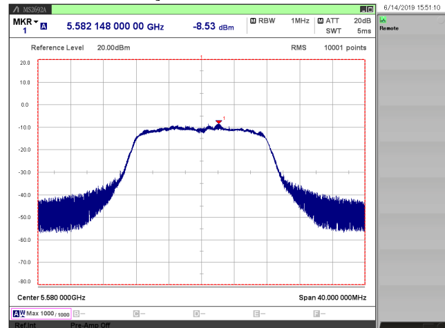
[ 802.11a/ 5580 MHz ]
