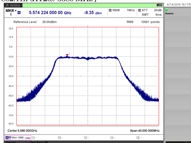
[ 802.11n (HT20)/ 5580 MHz ]
