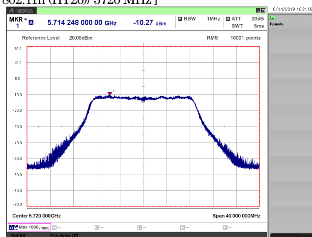
[ 802.11n (HT20)/ 5720 MHz ]
