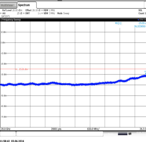
Band41_10MHz_QPSK_39700_1RB#0_20000~26500_20000~26500
