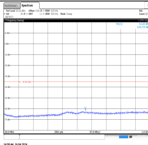
Band41_10MHz_QPSK_40620_1RB#0_30~1000_30~1000
