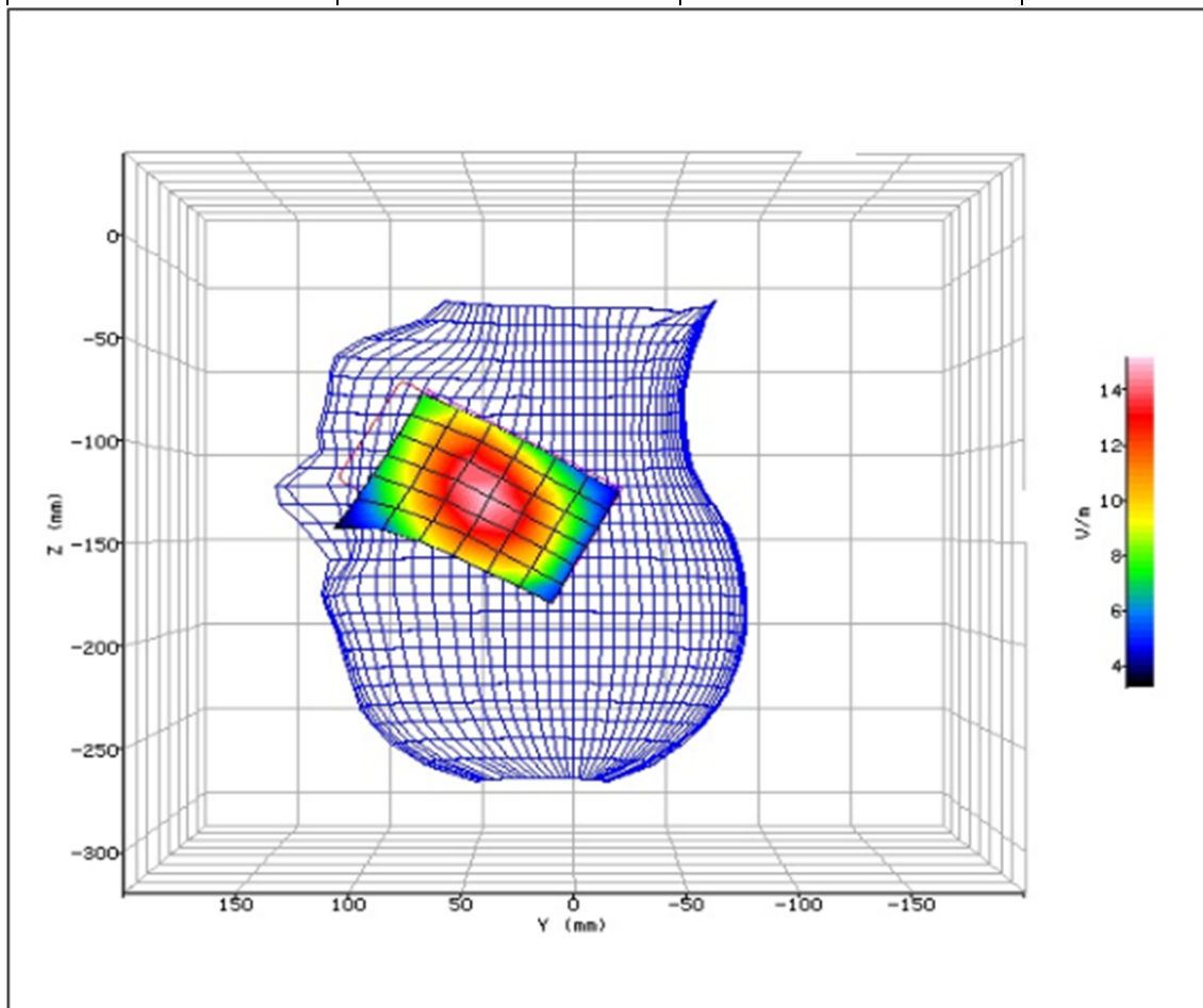
Figure 7: SAR Head Testing Results for the Sharp SHV31 Mobile Handset at 824.2MHz.
