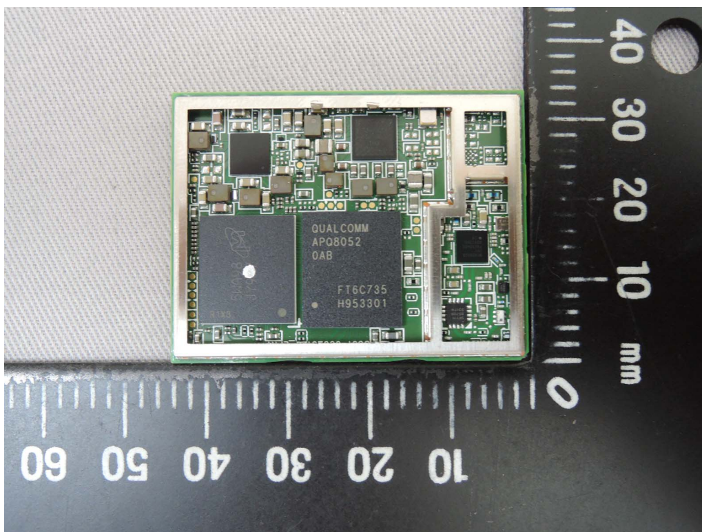
Internal View of EUT -2( Frey M1-0010)
