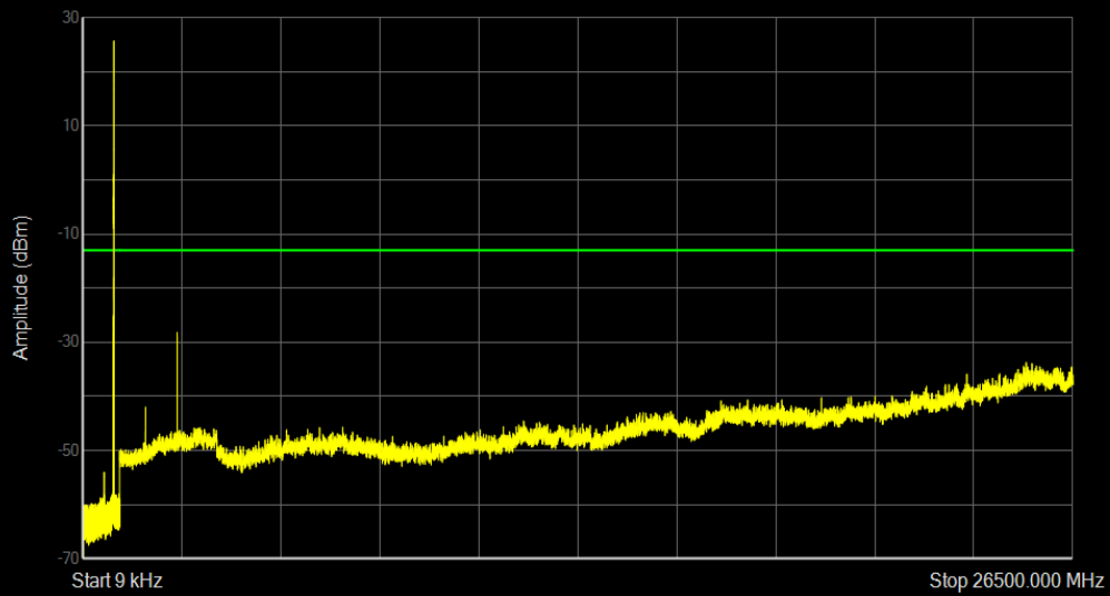
Band26(824-849) QPSK BW=3MHz Channel=27025 RB Size=1 Position=#0
