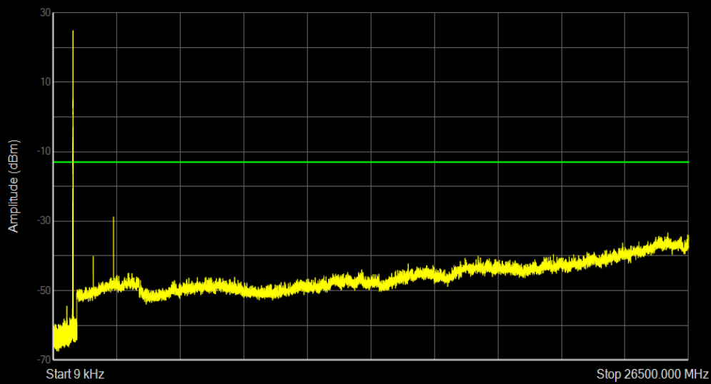
Band26(824-849) QPSK BW=5MHz Channel=27015 RB Size=1 Position=#0
