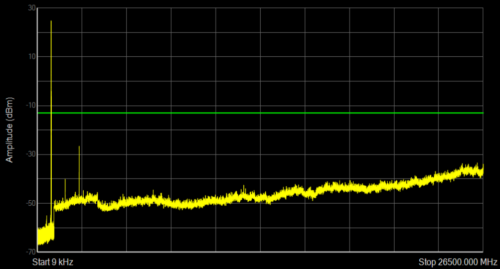
Band26(824-849) QPSK BW=5MHz Channel=26915 RB Size=1 Position=#0
