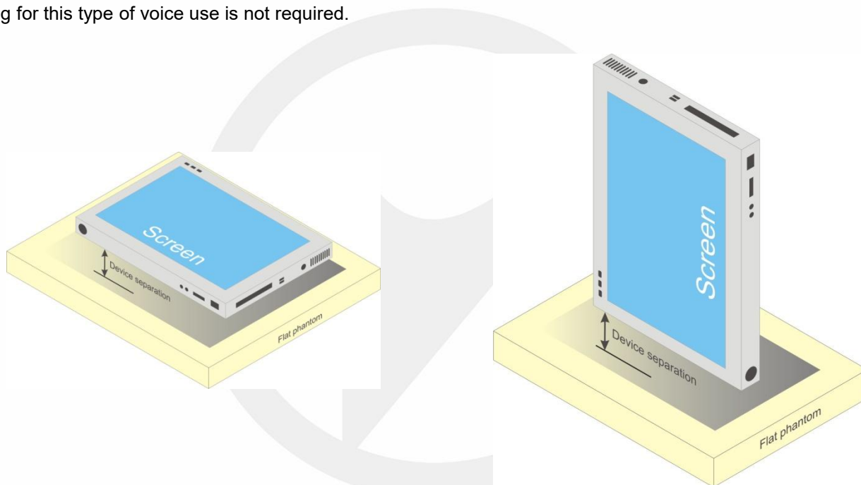
Fig-4.1 Illustration for Tablet Setup
