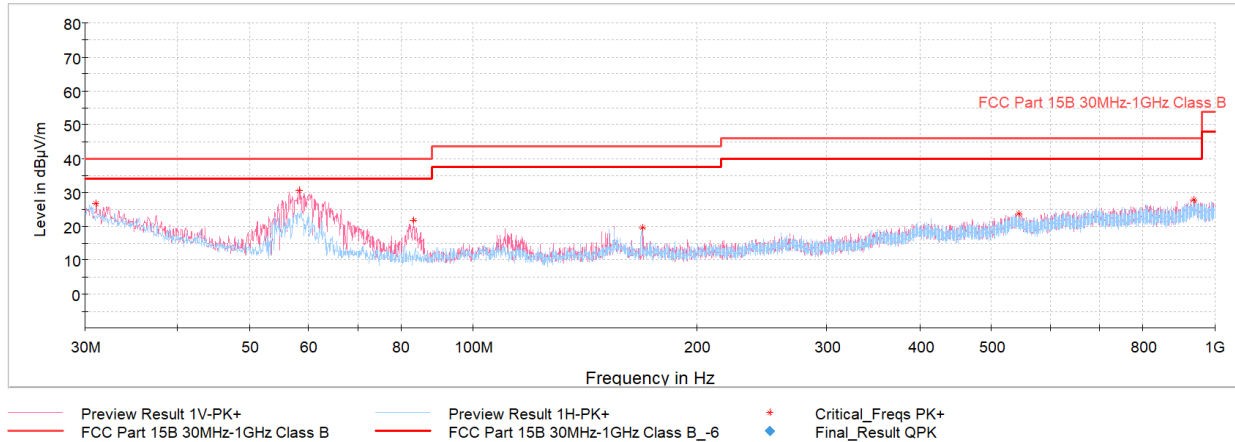
Plot 6-1. Radiated Emissions Pre-Scan 30MHz-1GHz
