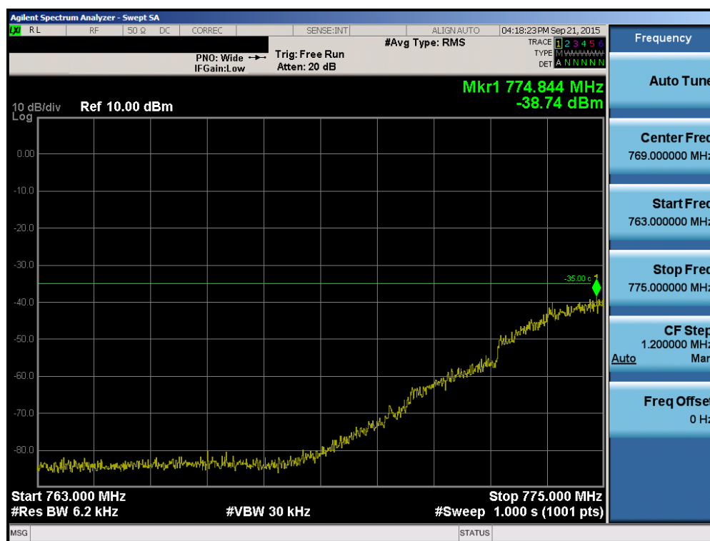
Plot 6-36. Lower Emission Mask Edge Plot (Band 13 – 5.0MHz QPSK – RB Size 25)
