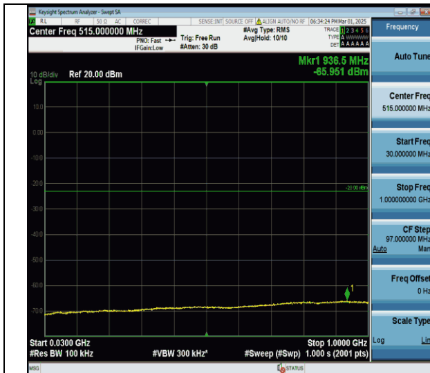
Band66-20MHz-QPSK-132572-1RB#0-30~1000-PASS
