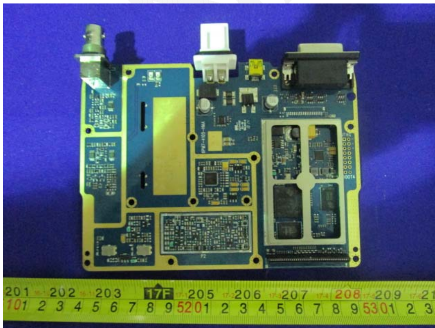
EUT –Main Board Top(Off Shielding) View
