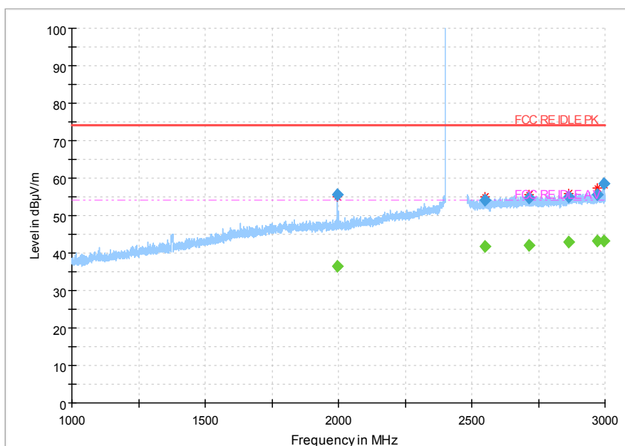
Fig.56 Radiated emission: 8DPSK, Ch0, 1GHz~3GHz
