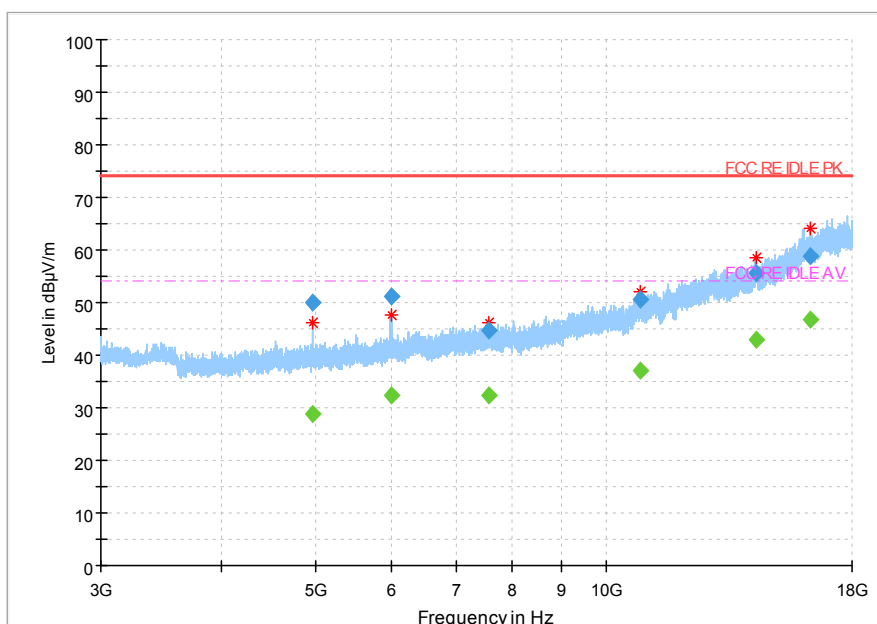
Fig.62 Radiated emission: 8DPSK, Ch0, 3GHz~18GHz
