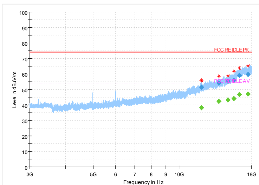
Fig.57 Radiated emission: 8DPSK, Ch0, 3GHz~18GHz
