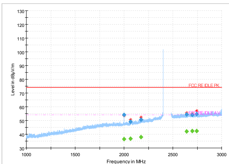
Fig.61 Radiated emission: 8DPSK, Ch0, 1GHz~3GHz
