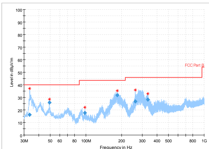
Fig.60 Radiated emission: 8DPSK, Ch0, 30MHz~1GHz
