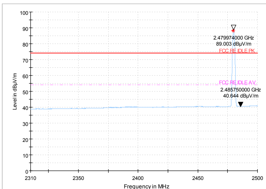
Fig.64 Radiated emission (Power): 8DPSK, high channel
