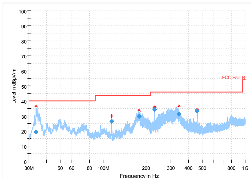
Fig.55 Radiated emission: 8DPSK, Ch0, 30MHz~1GHz
