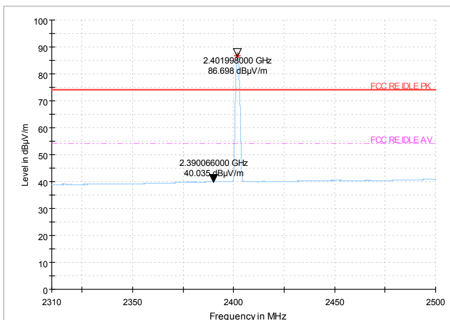
Fig.58 Radiated emission (Power): 8DPSK, low channel
