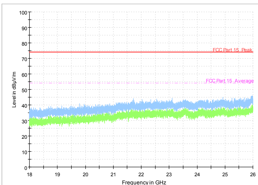
Fig.64 Radiated emission (Power): 8DPSK, high channel
