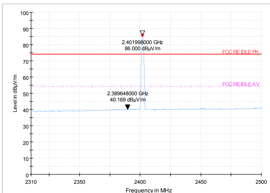
Fig.63 Radiated emission (Power): 8DPSK, low channel
