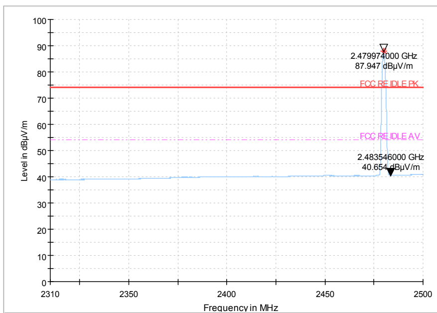
Fig.59 Radiated emission (Power): 8DPSK, high channel
