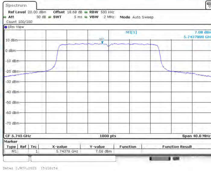
11AX20-CDD_Ant3_5745
