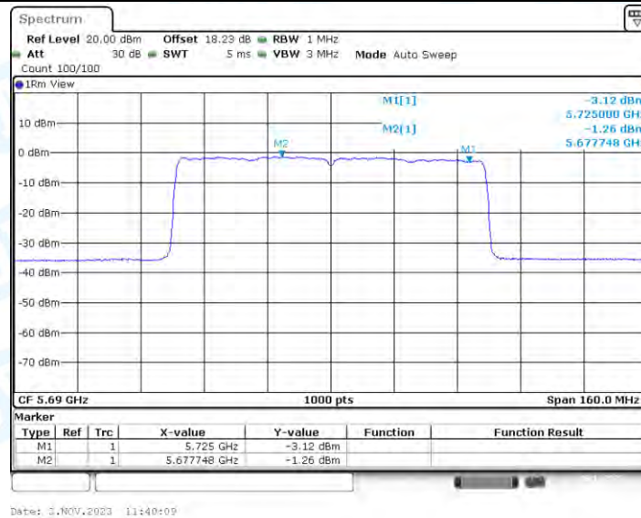
11AX80-CDD_Ant3_5690_UNII-2C
