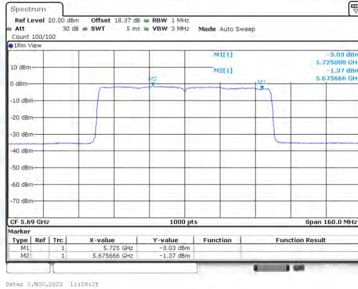
11AX80-CDD_Ant2_5690_UNII-2C
