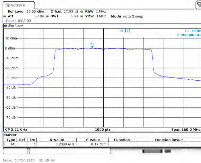
11AX80-CDD_Ant4_5210
