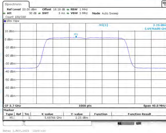
11AX20-CDD_Ant3_5700
