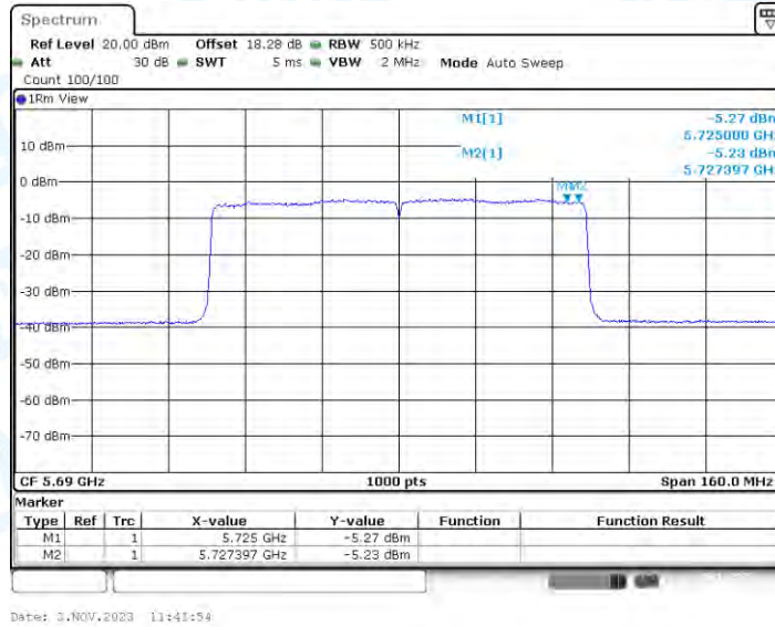
11AX80-CDD_Ant4_5690_UNII-3
