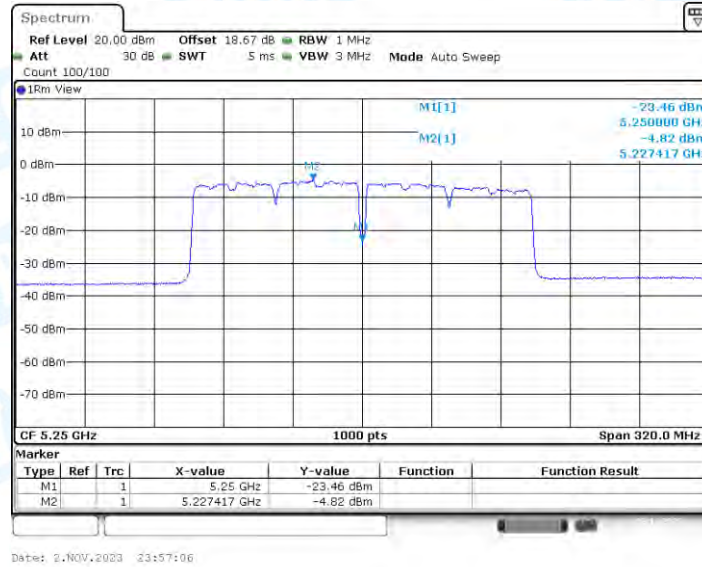
11AC160-CDD_Ant4_5250_UNII-1
