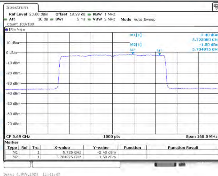
11AX80-CDD_Ant4_5690_UNII-2C
