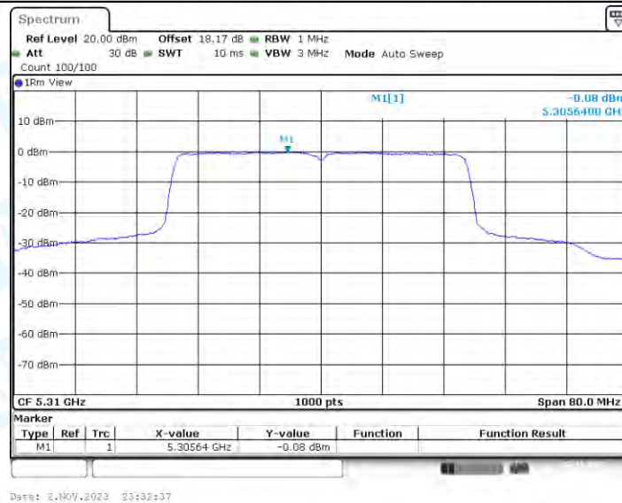
11AX40-CDD_Ant4_5310
