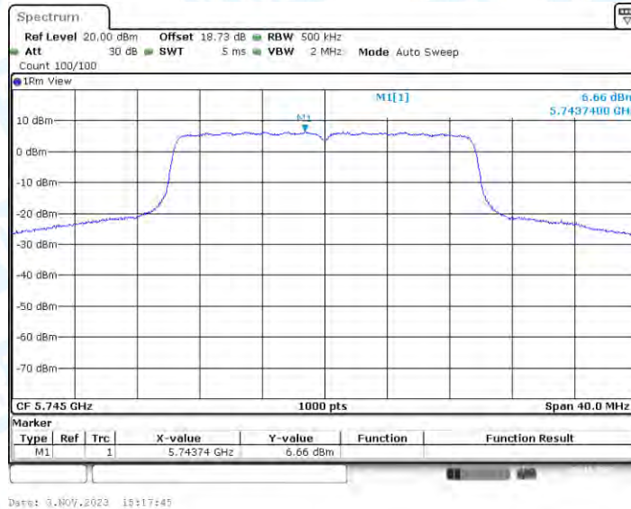
11AX20-CDD_Ant4_5745
