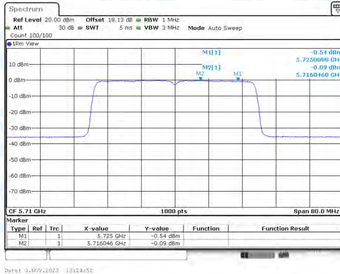
11AX40-CDD_Ant3_5710_UNII-2C
