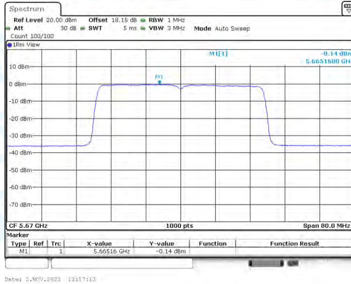
11AX40-CDD_Ant3_5670
