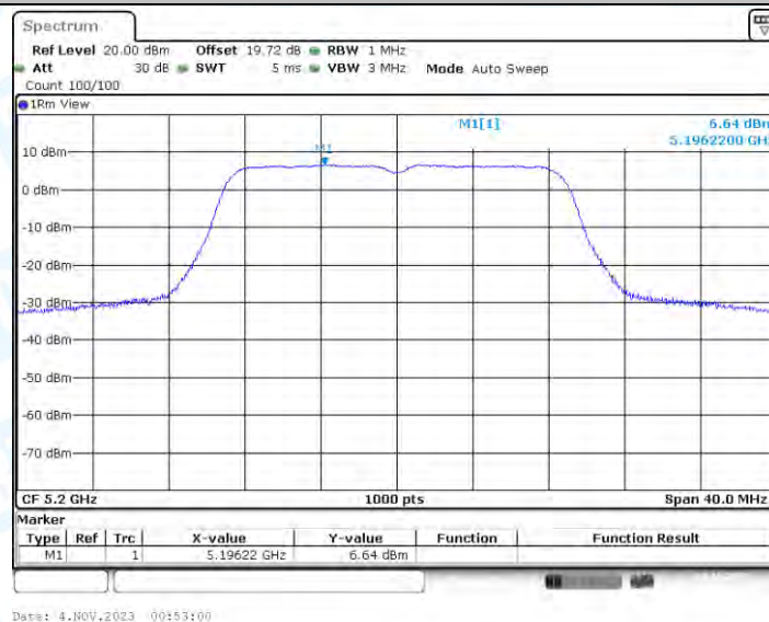
11N20-BF_Ant4_5200
