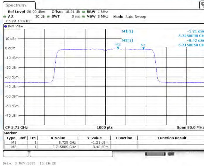
11AX40-CDD_Ant4_5710_UNII-2C
