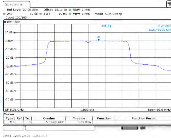
11AX40-CDD_Ant2_5310
