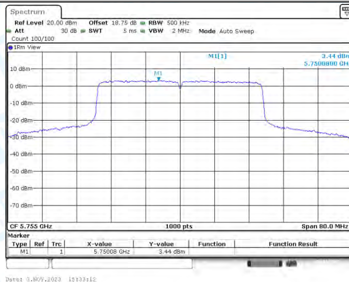
11AX40-CDD_Ant4_5755
