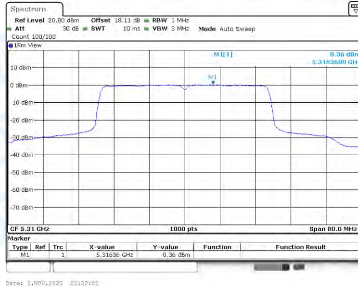
11AX40-CDD_Ant3_5310
