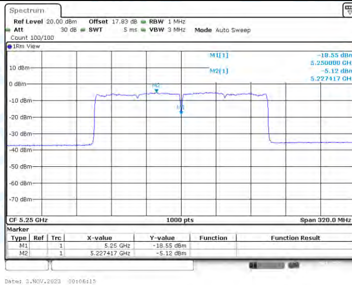
11AX160-CDD_Ant3_5250_UNII-1
