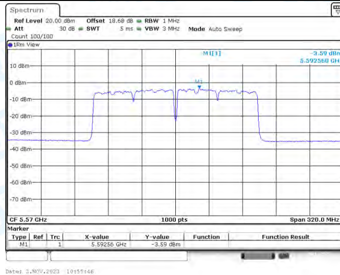
11AC160-CDD_Ant3_5570
