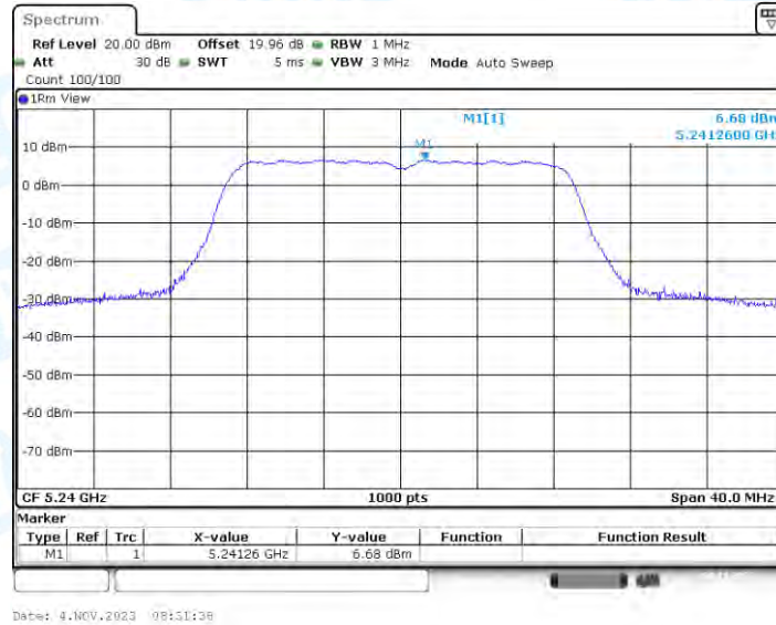
11N20-BF_Ant4_5240
