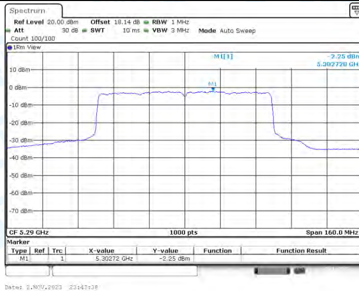
11AX80-CDD_Ant3_5290
