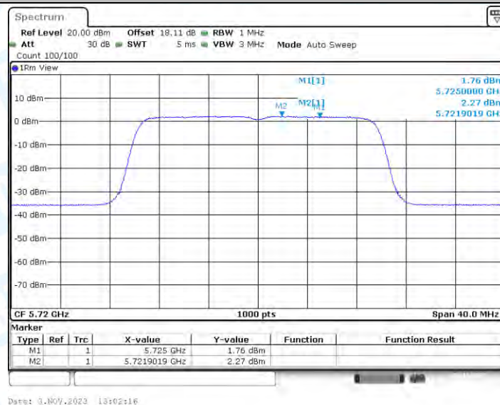
11AX20-CDD_Ant3_5720_UNII-2C
