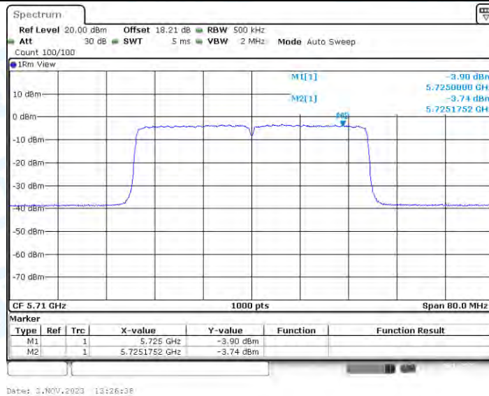
11AX40-CDD_Ant4_5710_UNII-3
