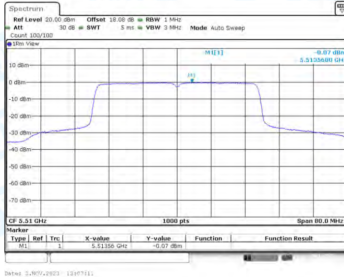
11AX40-CDD_Ant2_5510
