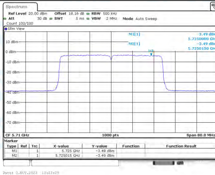
11AX40-CDD_Ant2_5710_UNII-3
