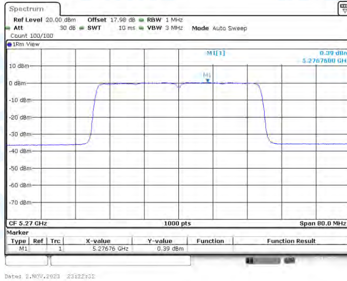
11AX40-CDD_Ant3_5270
