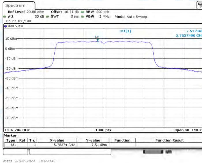
11AX20-CDD_Ant3_5785
