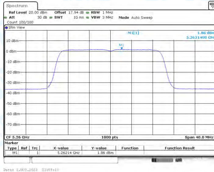
11AX20-CDD_Ant3_5260
