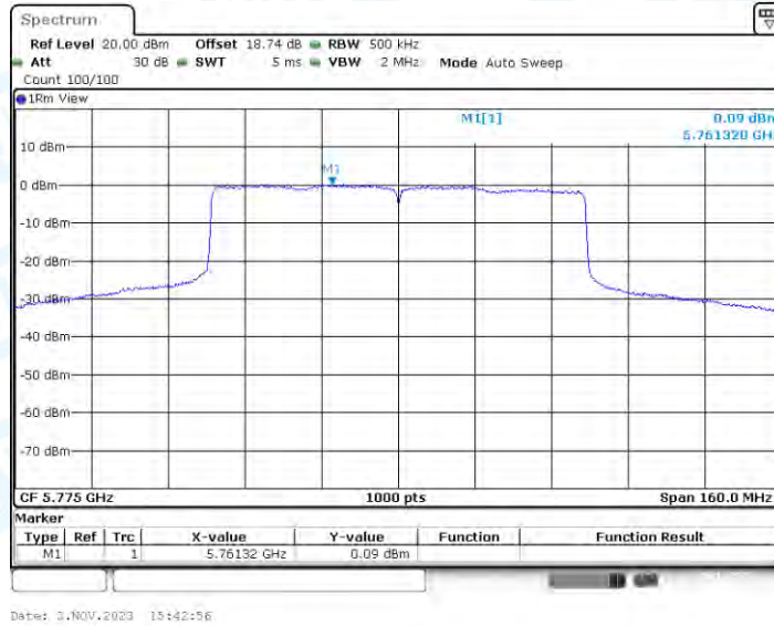
11AX80-CDD_Ant4_5775
