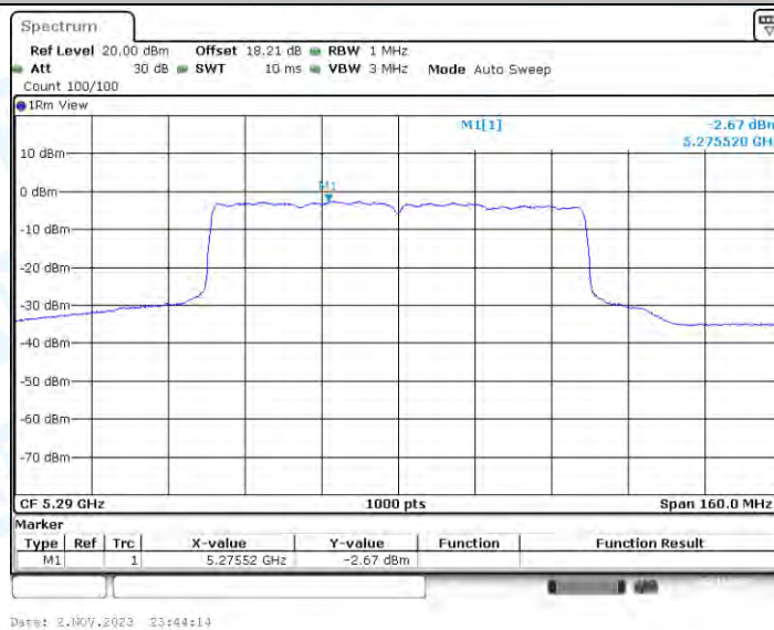
11AX80-CDD_Ant4_5290
