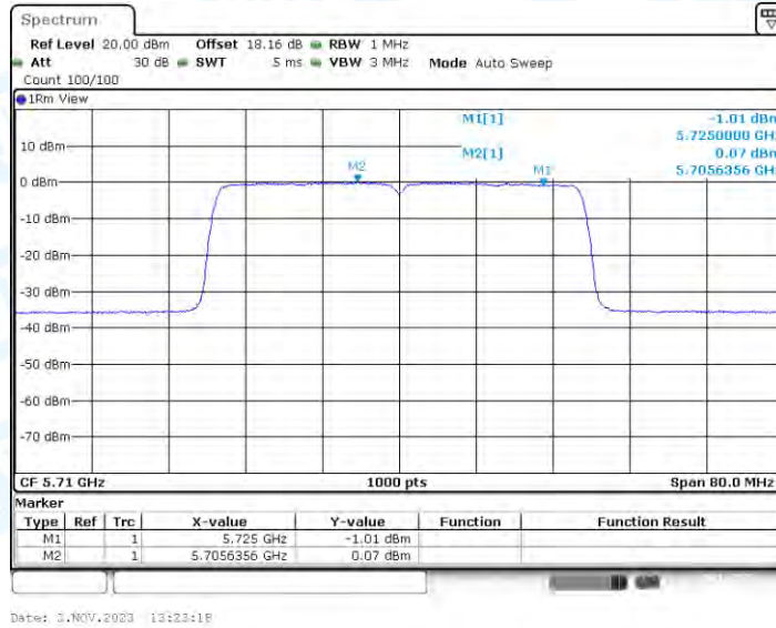
11AX40-CDD_Ant2_5710_UNII-2C
