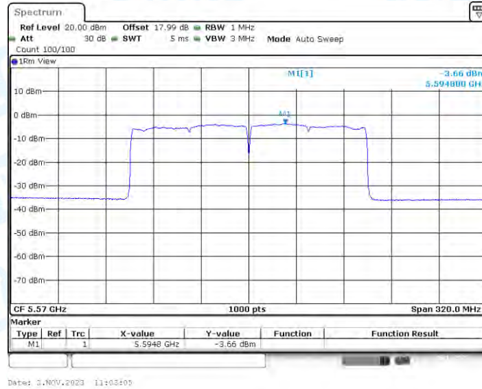
11AX160-CDD_Ant3_5570
