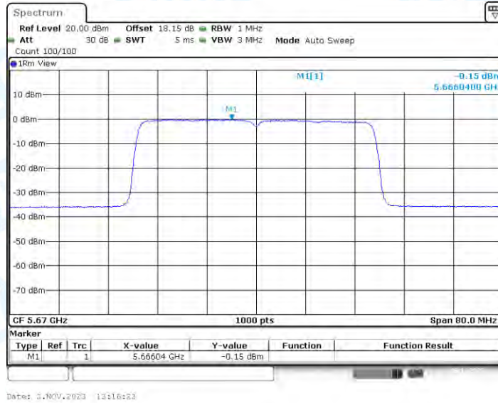
11AX40-CDD_Ant2_5670
