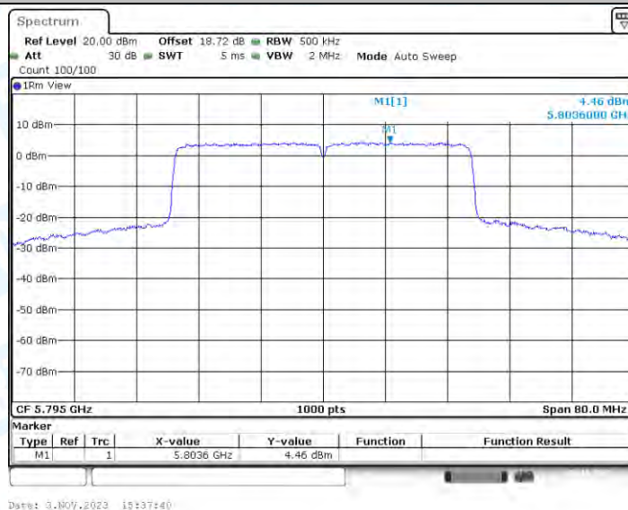
11AX40-CDD_Ant3_5795
