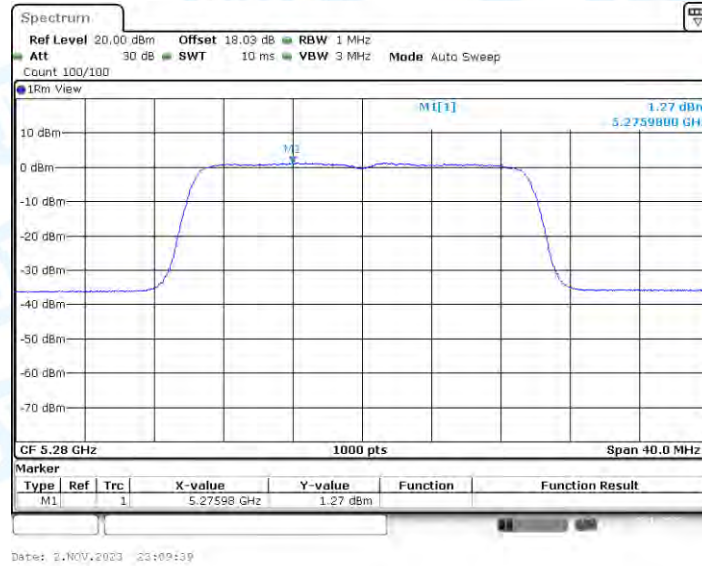
11AX20-CDD_Ant4_5280
