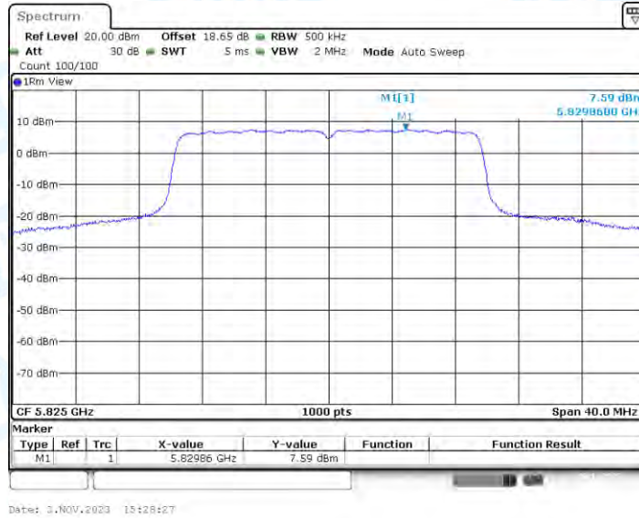
11AX20-CDD_Ant3_5825
