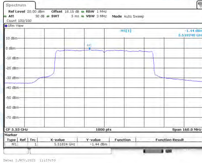
11AX80-CDD_Ant4_5530
