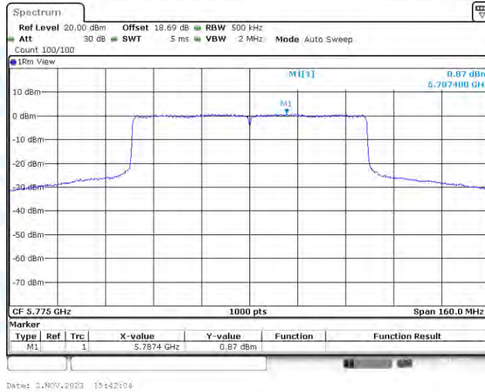
11AX80-CDD_Ant3_5775
