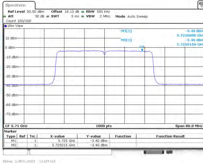
11AX40-CDD_Ant3_5710_UNII-3
