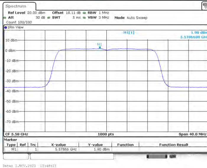
11AX20-CDD_Ant4_5580
