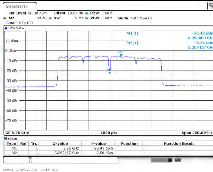
11AC160-CDD_Ant4_5250_UNII-2A
