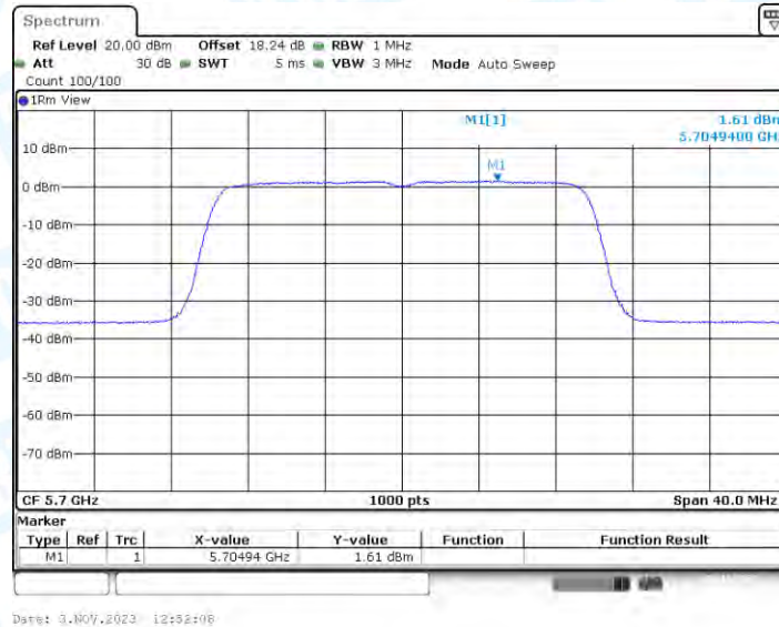
11AX20-CDD_Ant4_5700
