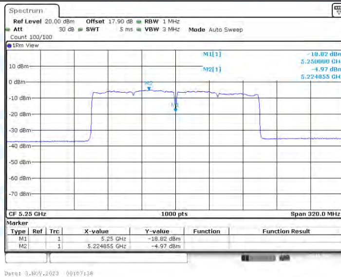
11AX160-CDD_Ant4_5250_UNII-1
