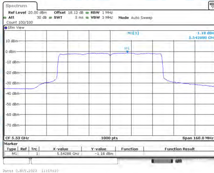
11AX80-CDD_Ant3_5530
