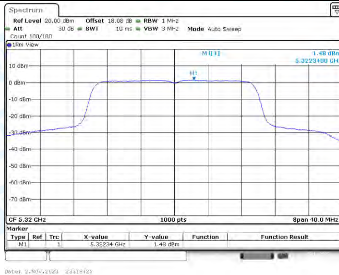
11AX20-CDD_Ant3_5320
