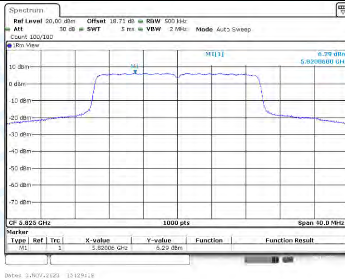
11AX20-CDD_Ant4_5825
