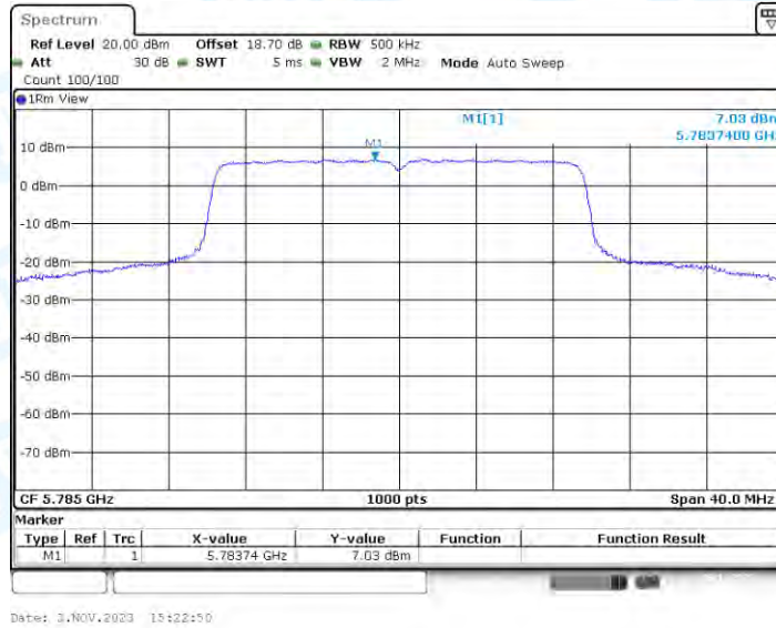
11AX20-CDD_Ant2_5785
