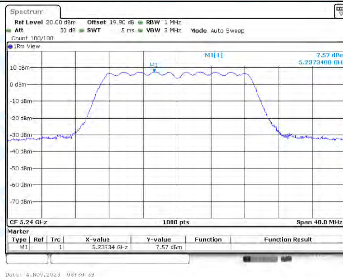
11N20-BF_Ant3_5240
