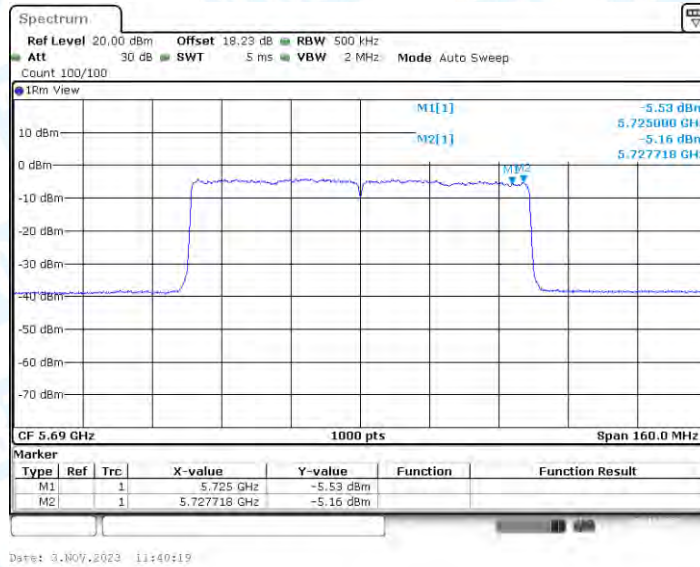
11AX80-CDD_Ant3_5690_UNII-3
