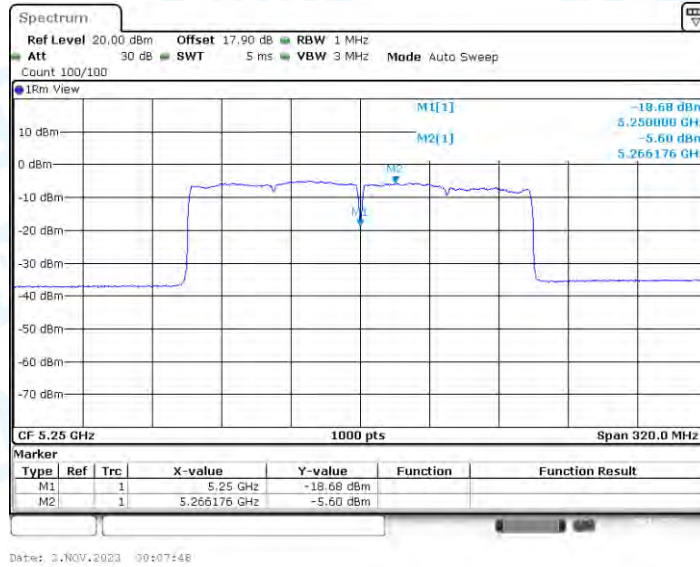
11AX160-CDD_Ant4_5250_UNII-2A
