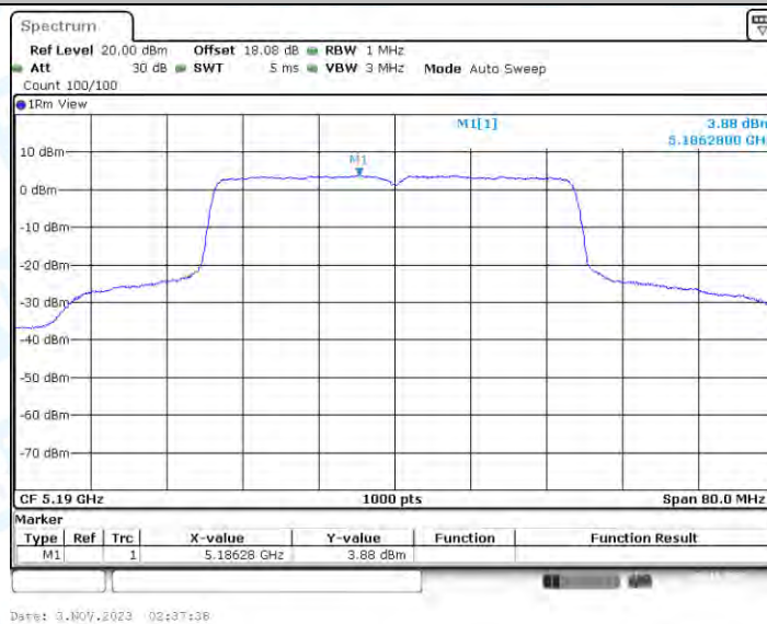
11AX40-CDD_Ant4_5190
