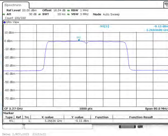
11AX40-CDD_Ant4_5270
