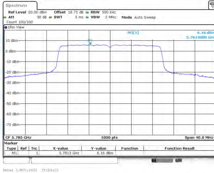
11AX20-CDD_Ant4_5785
