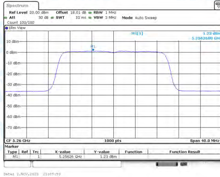
11AX20-CDD_Ant4_5260
