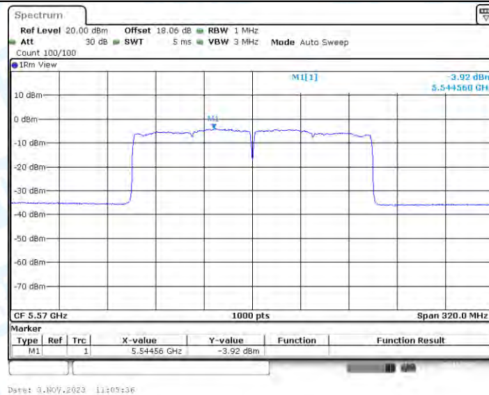
11AX160-CDD_Ant4_5570
