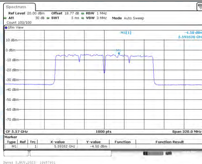
11AC160-CDD_Ant4_5570
