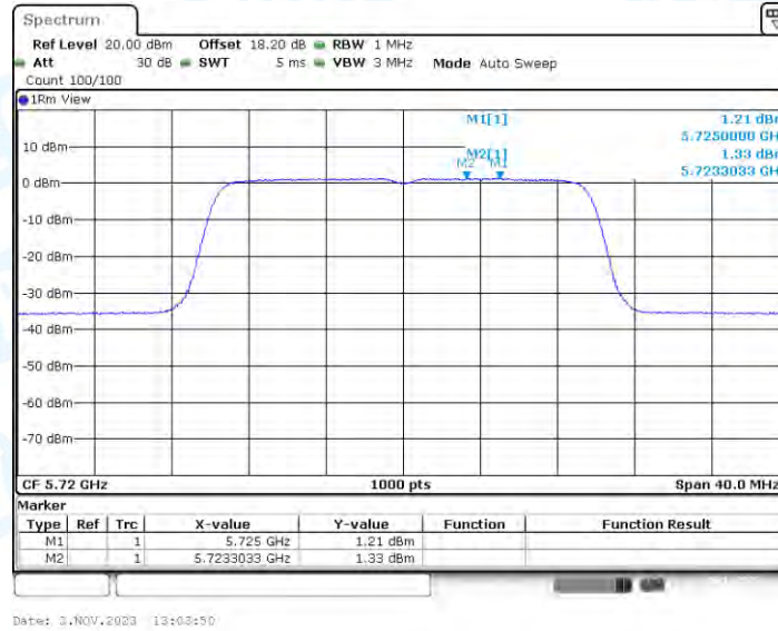
11AX20-CDD_Ant4_5720_UNII-2C
