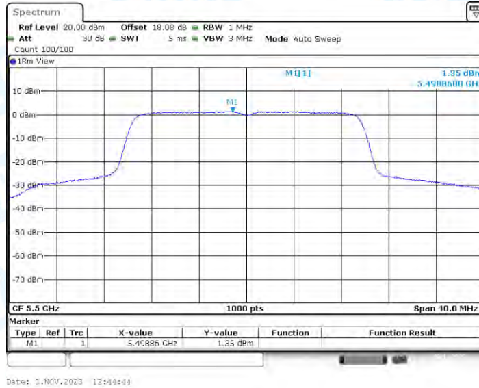
11AX20-CDD_Ant4_5500
