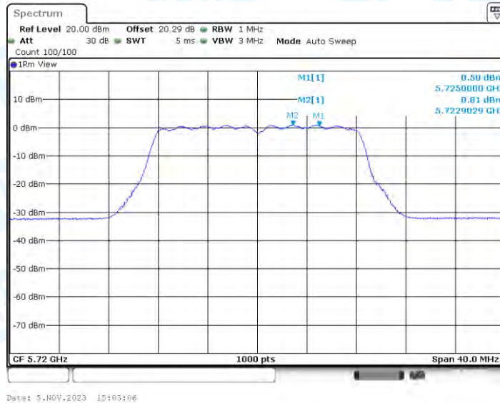
11A-BF_Ant4_5720_UNII-2C
