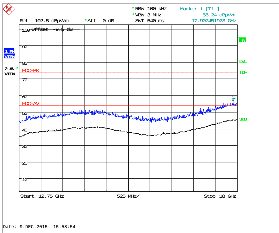
BTLE Channel 19 : 12.75 GHz to 18 GHz
