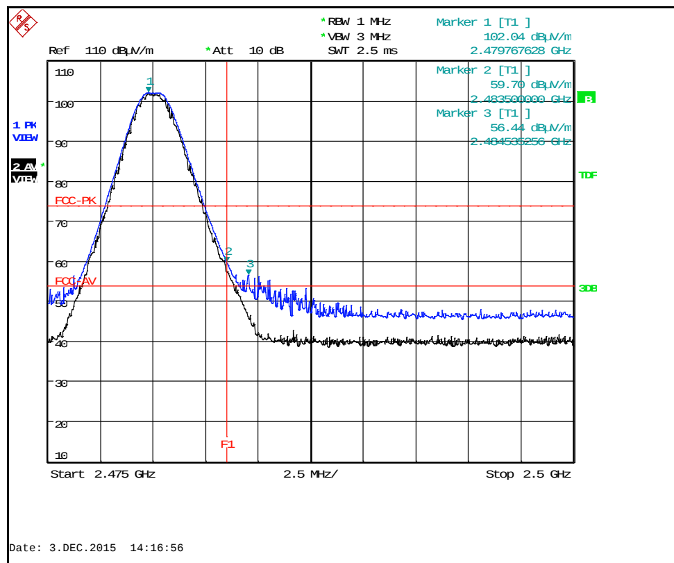
BTLE Channel 39 : Upper Band Edge
