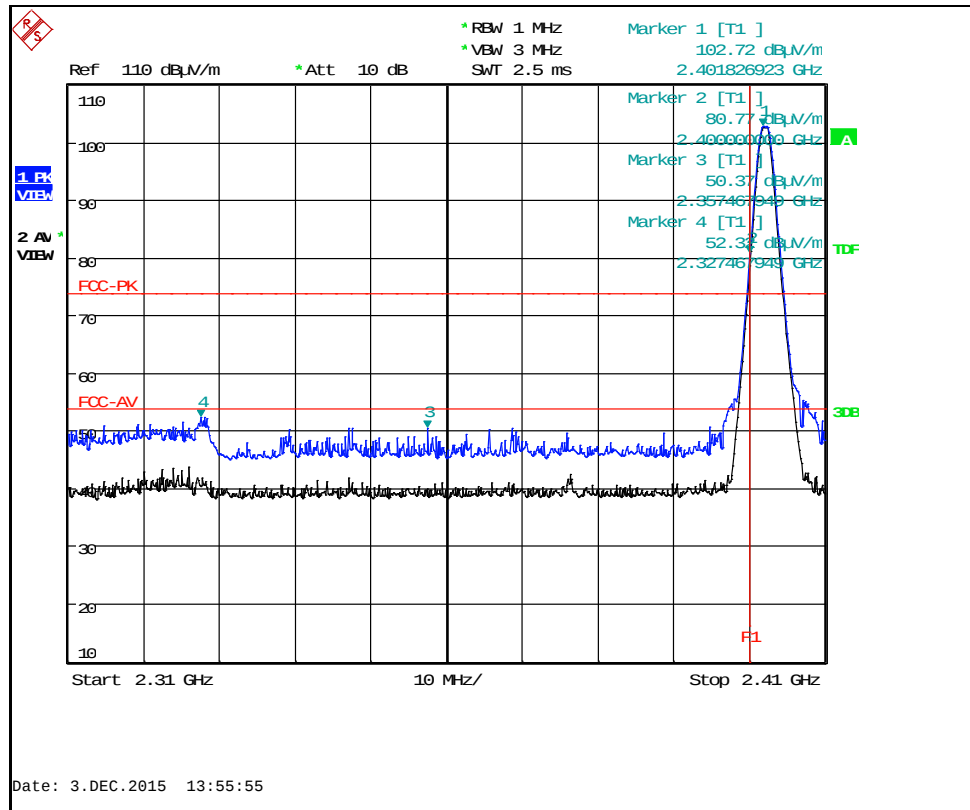
BTLE Channel 1 : Lower Band Edge
