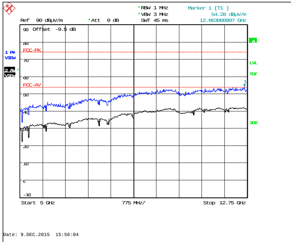
BTLE Channel 19 : 5 GHz to 12.75 GHz
