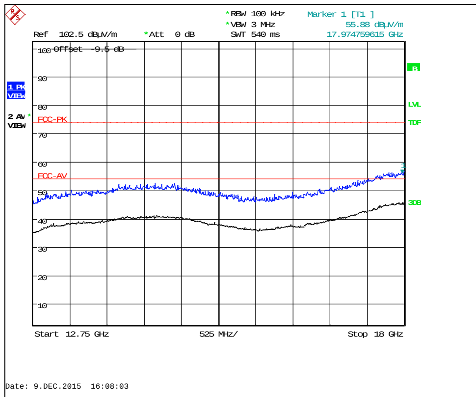
BTLE Channel 39 : 12.75 GHz to 18 GHz
