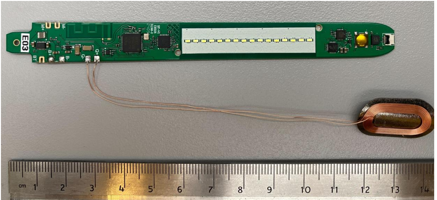
Coil Antenna is receive only
