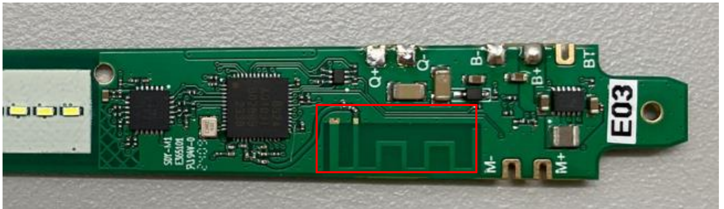
Top with Antenna highlighted in Red
