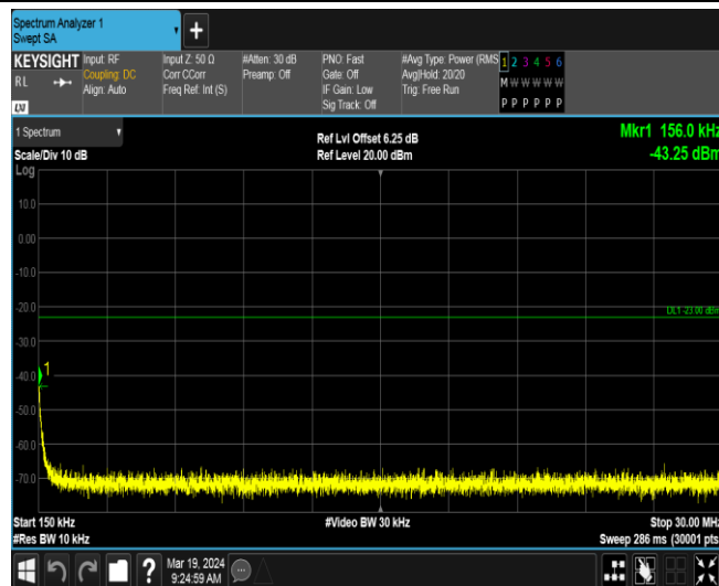
Band4-1513-5-0.15~30MHz
