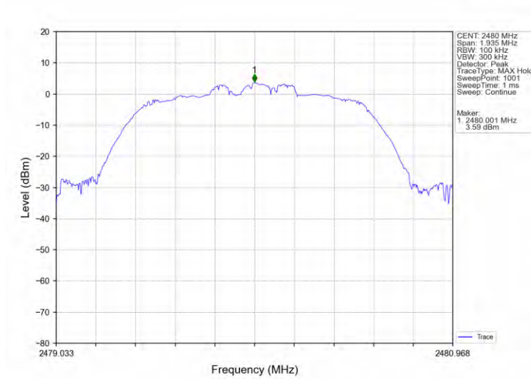
Pi/4DQPSK_2DH5_HCH_2480MHz_Ant1_NTNV
