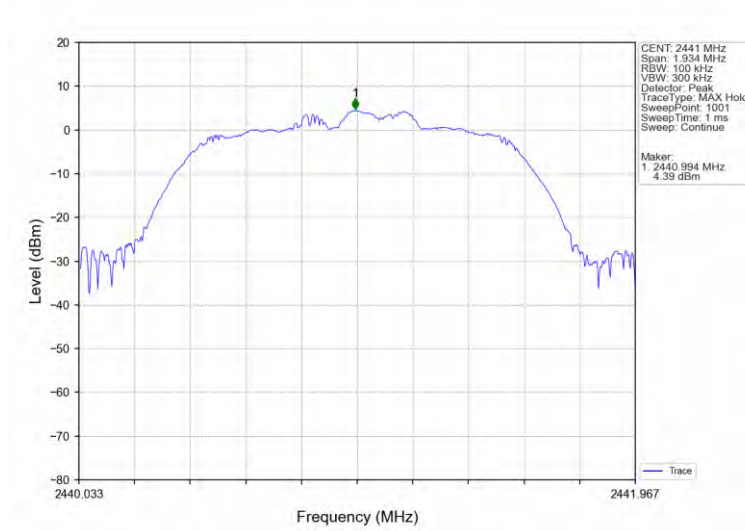
Pi/4DQPSK_2DH5_MCH_2441MHz_Ant1_NTNV
