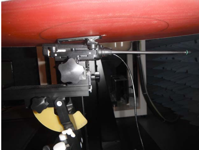
Back side of EUT in parallel to the phantom with the belt-clip (M/N: MB-133) in contact, attached HS-94 Ear-hook type
