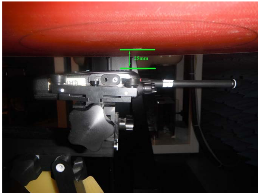
< FA-SC61VC cut antenna with the length of 133mm >
