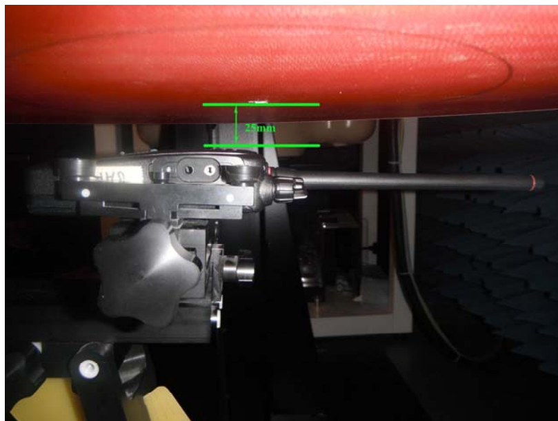
< FA-SC55V: 150MHz~174MHz; Red Ring>
