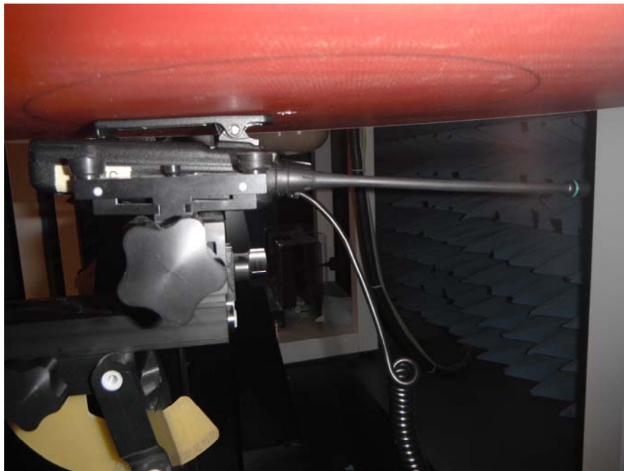
Back side of EUT in parallel to the phantom with the belt-clip (M/N: MB-133) in contact, attached HS-168LWP Speaker Microphone
