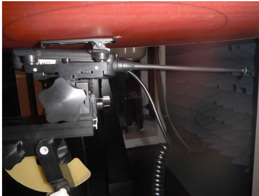
Back side of EUT in parallel to the phantom with the belt-clip (M/N: MB-133) in contact, attached HS-159LA Speaker Microphone
