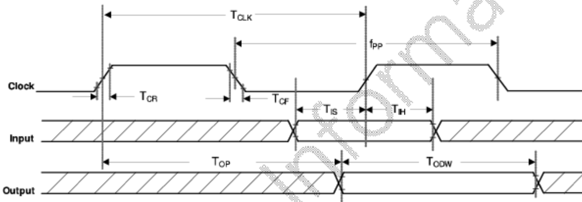
Figure 6: SDIO protocol timing diagram – SDR104 mode (208 MHz)
