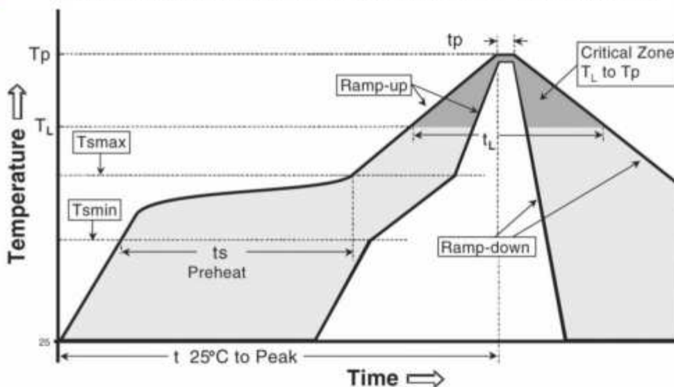
Figure 15: Reflow profile
