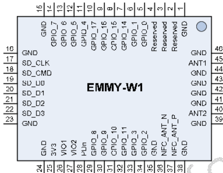
Figure 11: Pin assignment
