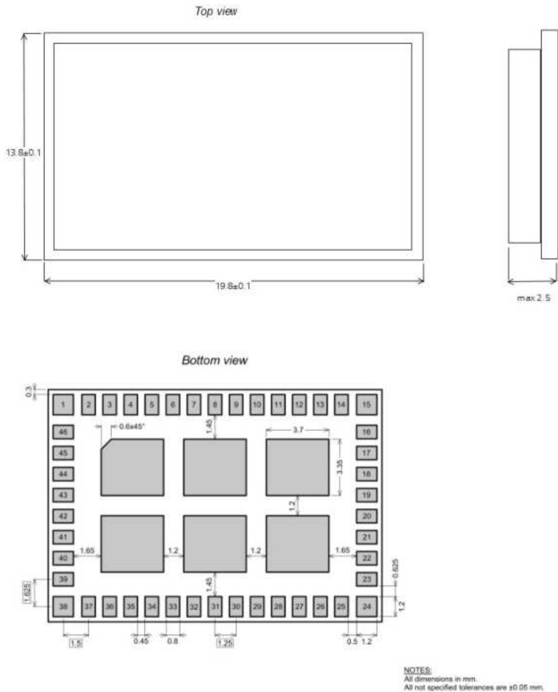
Figure 12: Physical dimensions
