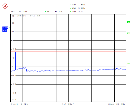
LTE Band 4 1.4MHz CH-Middle 1GHz ~20GHz
