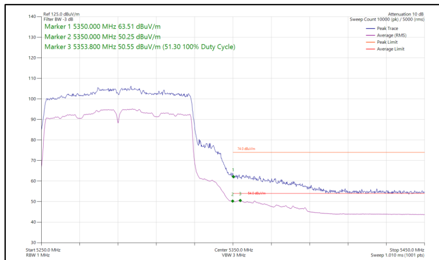
Figure 176 - 802.11ac VHT80, SISO, Core 0 - 5290 MHz Band Edge Frequency 5350 MHz
