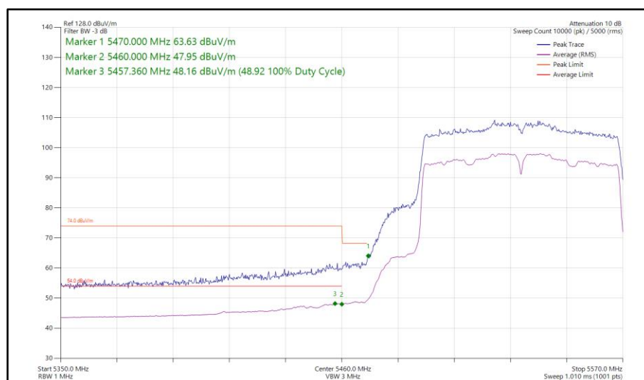
Figure 188 - 802.11ac VHT80, SISO, Core 1 - 5530 MHz Band Edge Frequency 5460 MHz
