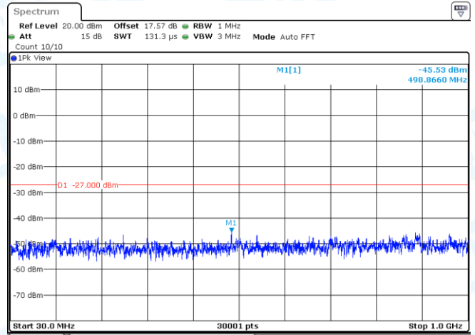
11AC20MIMO-Ant2-5240-30~1000-PASS
