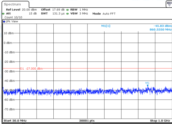
11N40MIMO-Ant1-5795-30~1000-PASS
