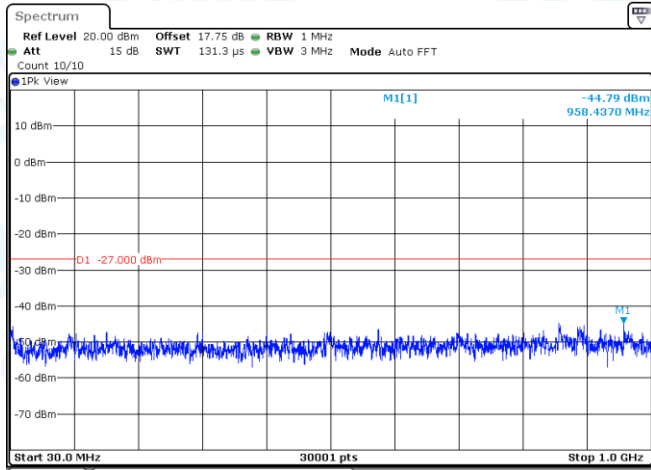
11AX40MIMO-Ant1-5755-30~1000-PASS
