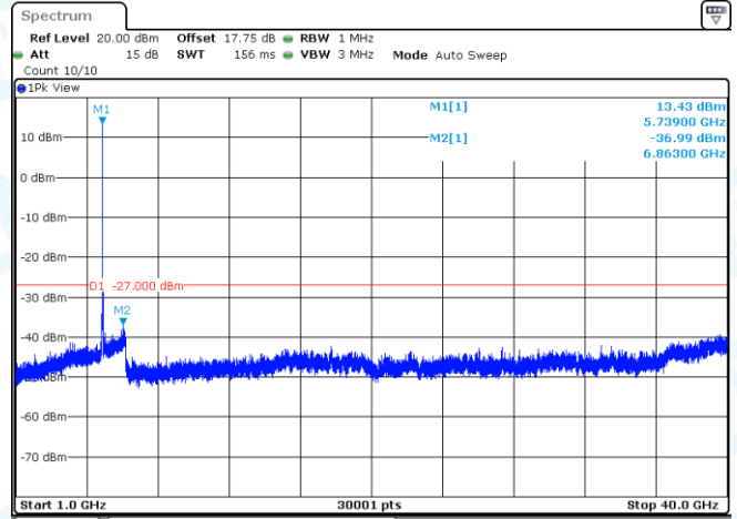
11AX20MIMO-Ant2-5745-1000~40000-PASS
