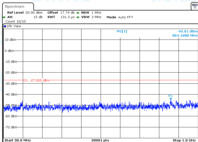
11AC20MIMO-Ant1-5825-30~1000-PASS
