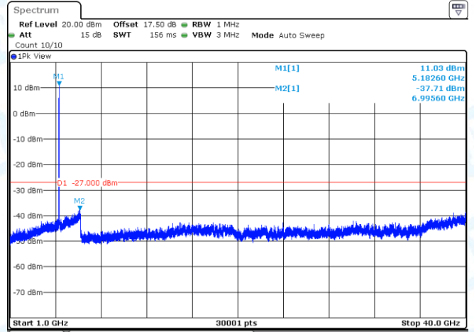
11AC20MIMO-Ant2-5180-1000~40000-PASS
