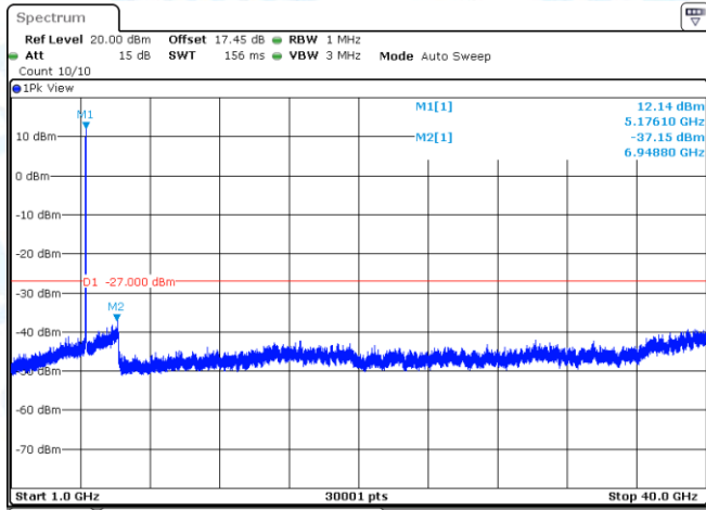
11AX20MIMO-Ant1-5180-1000~40000-PASS
