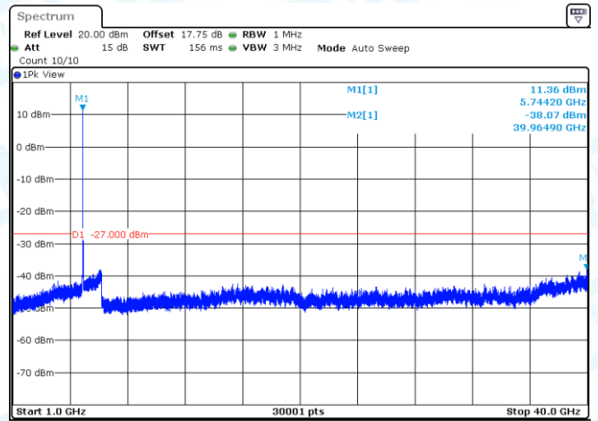
11AC20MIMO-Ant2-5745-1000~40000-PASS
