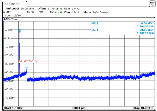
11AC40MIMO-Ant2-5190-1000~40000-PASS
