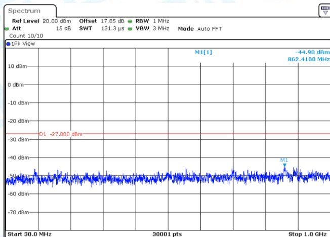
11AC20MIMO-Ant2-5825-30~1000-PASS
