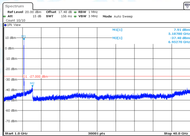
11AX40MIMO-Ant2-5190-1000~40000-PASS
