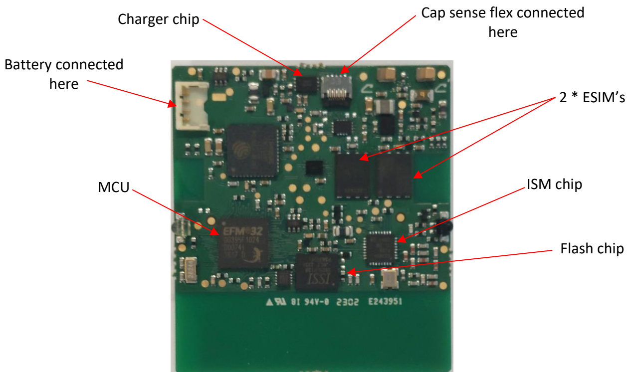
Figure 2 – Smart Tag 5 XB PCBA rear-side
