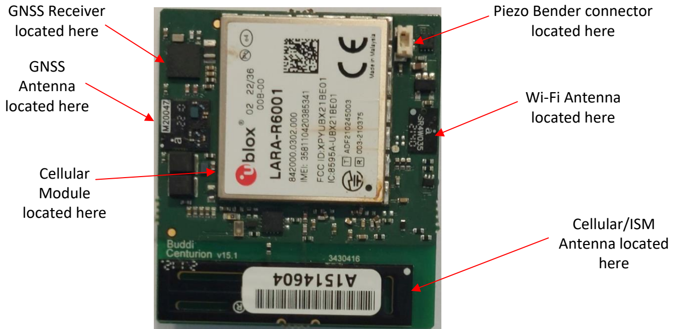
Figure 1 – Smart Tag 5 XB PCBA top-side
