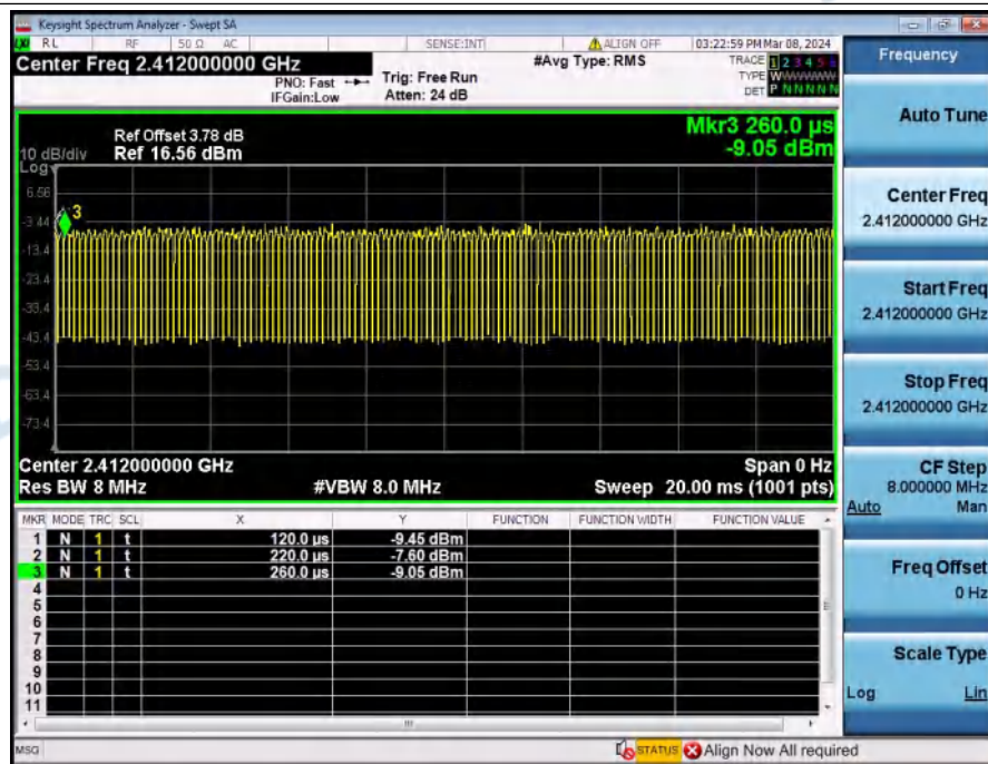
Duty_Cycle_NVNT_ANT1_802_11n(HT20)_2412
