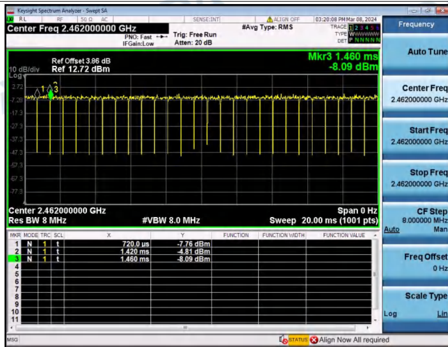
Duty_Cycle_NVNT_ANT1_802_11g_2462
