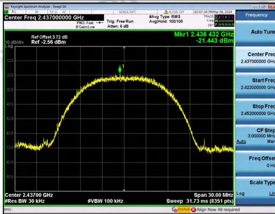
Power_Spectral_Density_NVNT_ANT1_802_11b_2437
