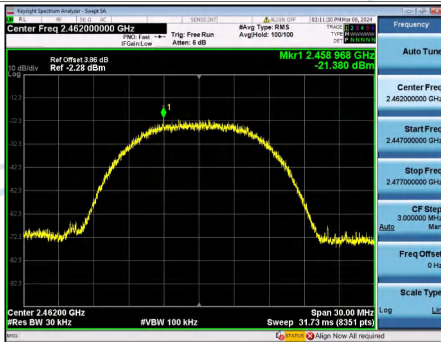
Power_Spectral_Density_NVNT_ANT1_802_11b_2462
