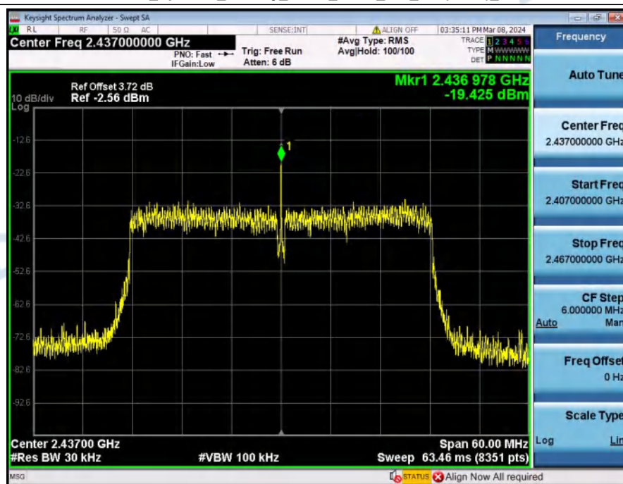
Power_Spectral_Density_NVNT_ANT1_802_11n(HT40)_2437
