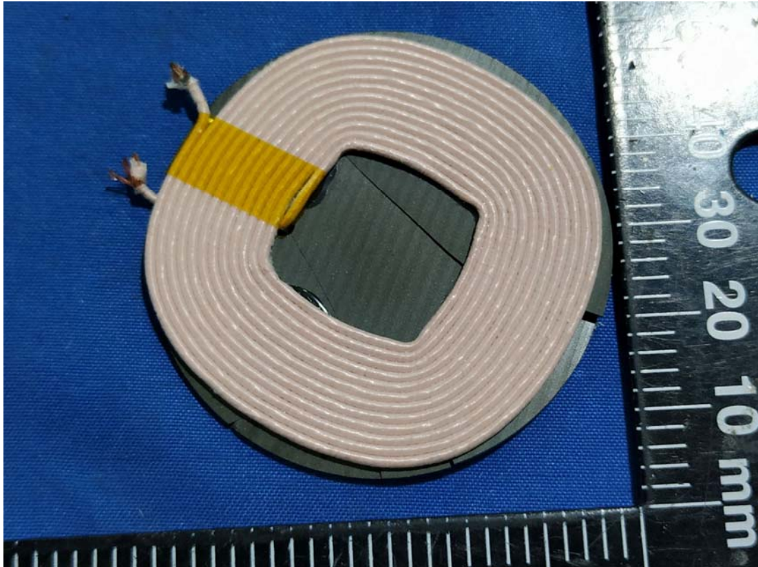
Coil Antenna
