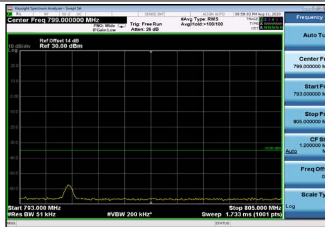
HighRange_FDD13_10MHz_782_fullRB _High_QPSK
