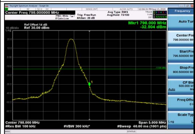
HighRange_FDD14_10MHz_793_OneRB _high_Q16
