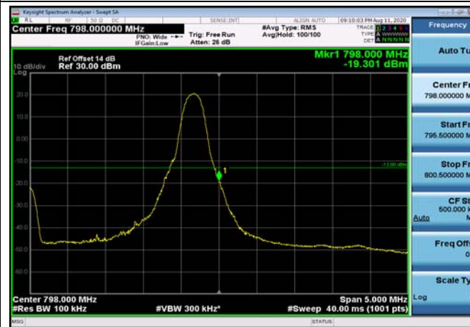
HighRange_FDD14_5MHz_795.5_fullRB _High_QPSK
