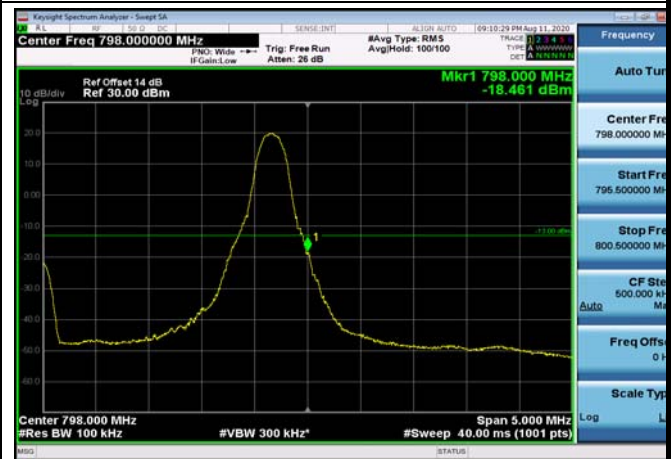
HighRange_FDD14_5MHz_795.5_fullRB _High_Q16
