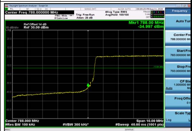
LowRange_FDD14_10MHz_793_fullRB _Low_Q16
