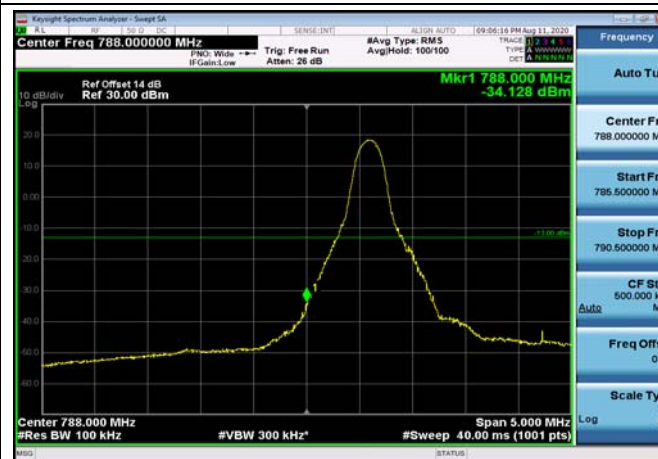
LowRange_FDD14_10MHz_793_fullRB _Low_QPSK
