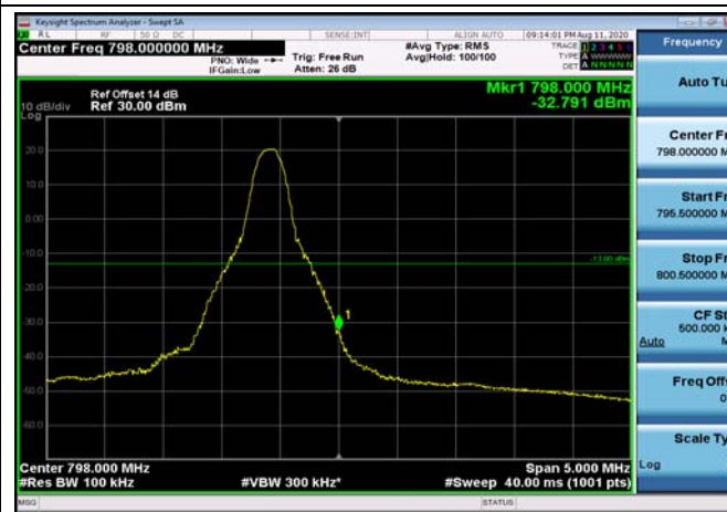
HighRange_FDD14_10MHz_793_OneRB _high_QPSK
