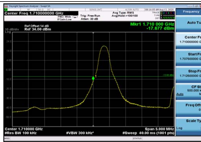
LowRange_FDD66_5MHz_1712.5_OneRB _low_QPSK
