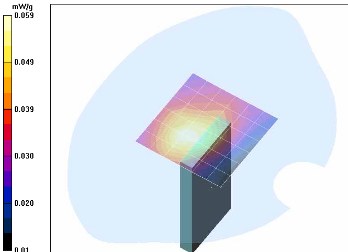
Fig. 6: SAR distribution for GPRS 850, channel 190, HP Omnibook XE2, position 3 (19.09.2005; Ambient Temperature: 21.2° C; Liquid Temperature: 20.5° C).
