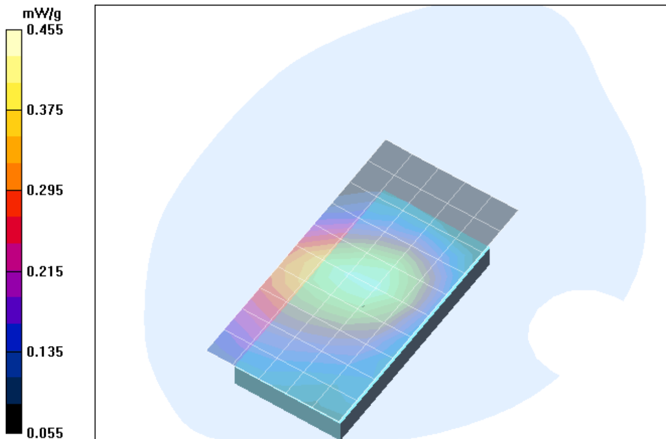
Fig. 5: SAR distribution for GPRS 850, channel 190, HP Omnibook XE2, position 2. (19.09.2005; Ambient Temperature: 21.2° C; Liquid Temperature: 20.5° C).
