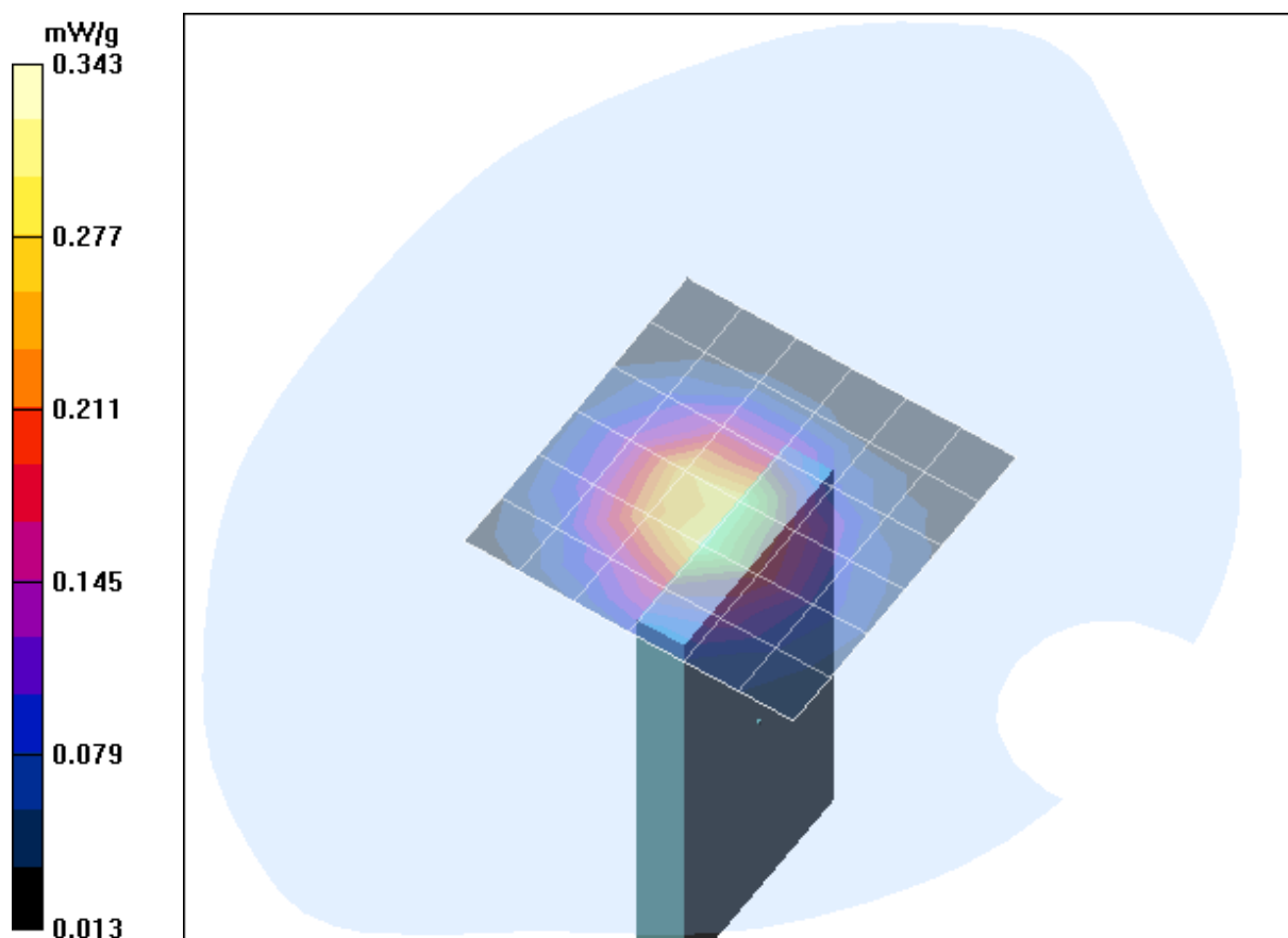
Fig. 18: SAR distribution for GPRS 1900, channel 661, HP Omnibook XE3, position 5. (20.09.2005; Ambient Temperature: 21.9° C; Liquid Temperature: 21.0° C).
