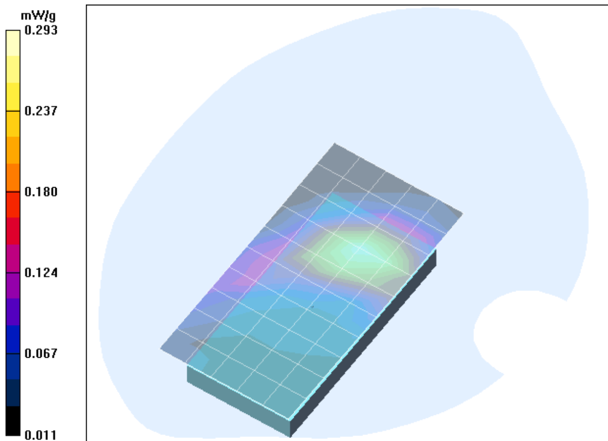
Fig. 13: SAR distribution for GPRS 1900, channel 661, HP Omnibook XE2, position 1. (20.09.2005; Ambient Temperature: 21.6° C; Liquid Temperature: 20.8° C).
