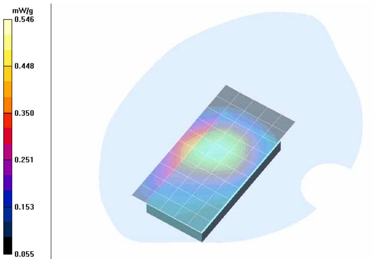
Fig. 7: SAR distribution for GPRS 850, channel 190, HP Omnibook XE3, position 1. (19.09.2005; Ambient Temperature: 21.8° C; Liquid Temperature: 20.7° C).
