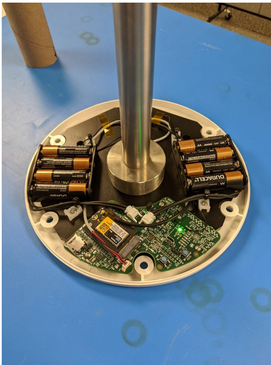
Figure 2: Main PCB Top Side
