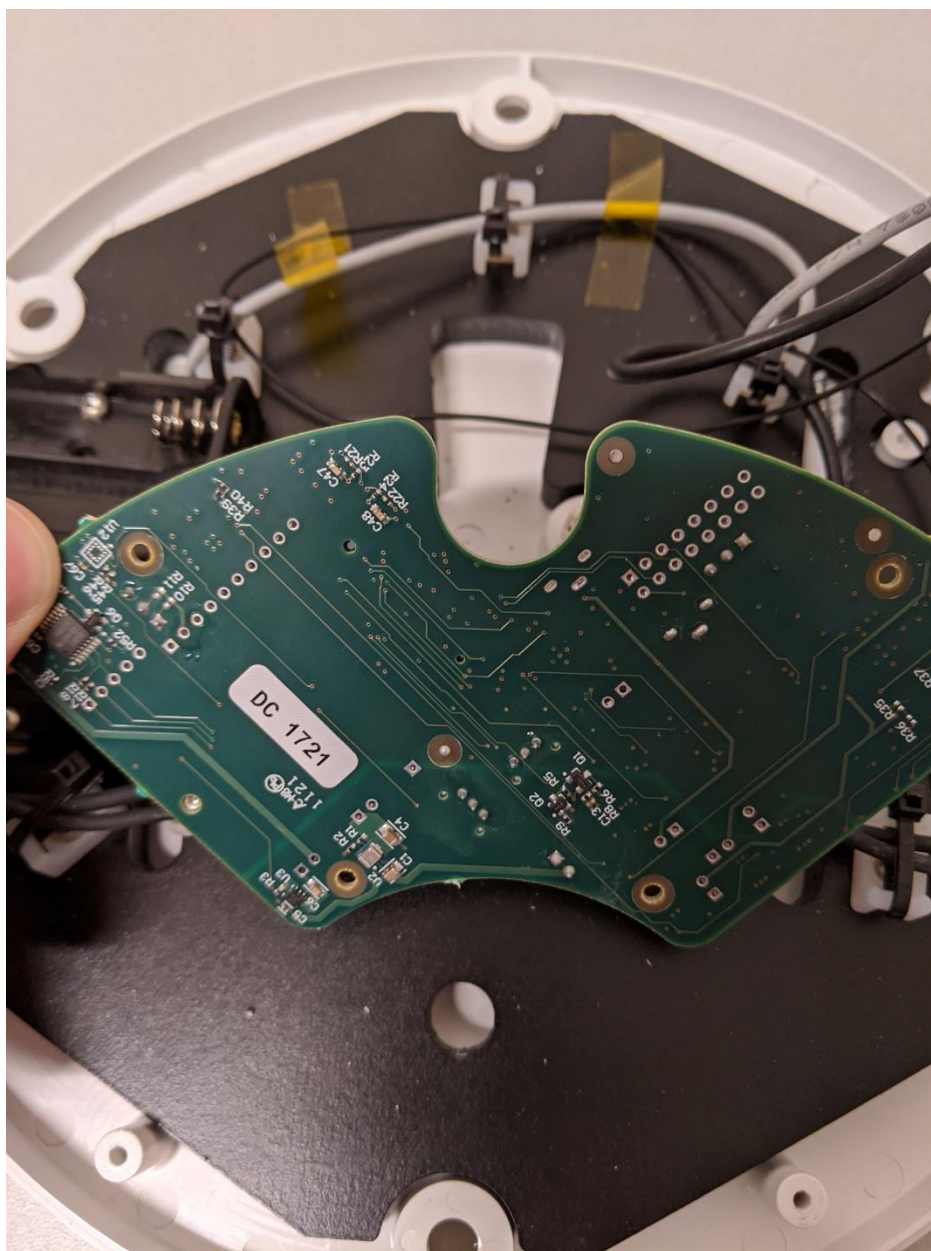
Figure 3: Main PCB Bottom Side
