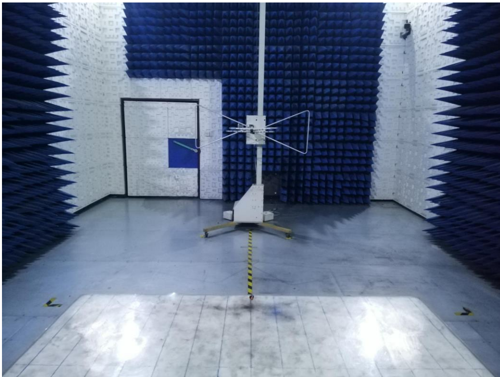
RADIATED EMISSION TEST SETUP BELOW 1GHz - Right
