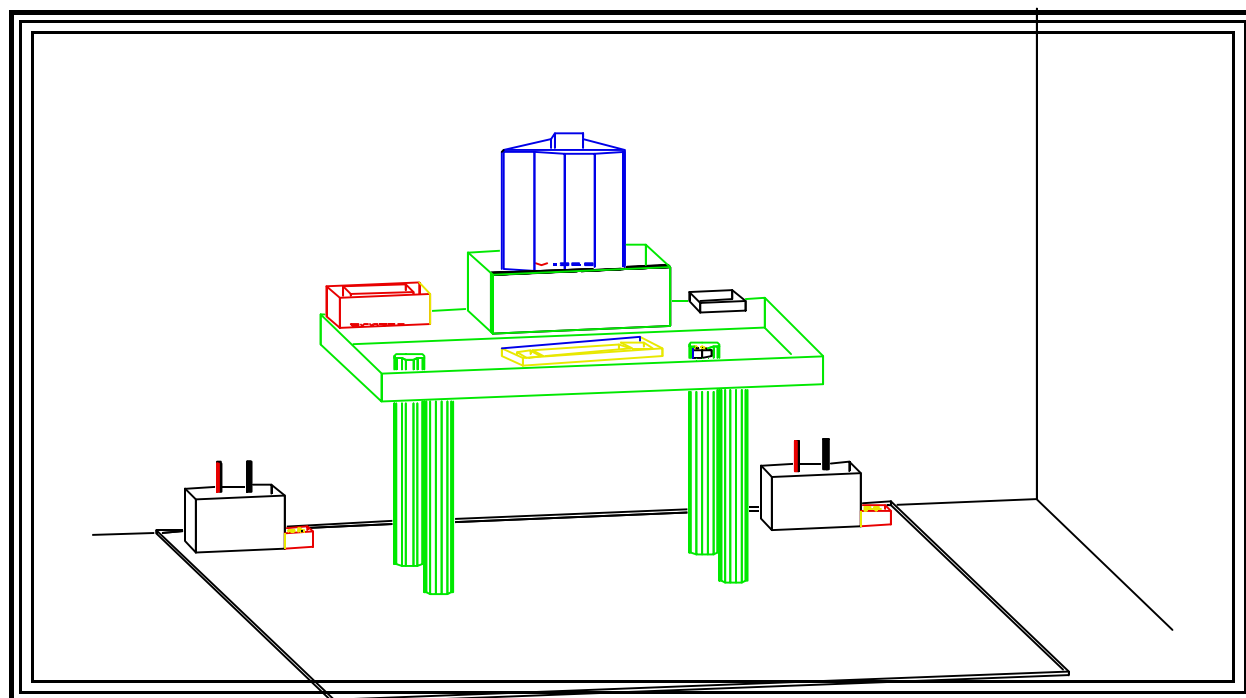
Fig. 10. System Setup. (Please see "Attachment F - Test Photographs" for actual system test set-up.)
