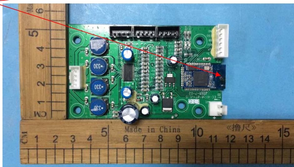
PCB Antenna
