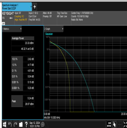
Band4-15MHz-QPSK-20325-1RB#0-PASS
