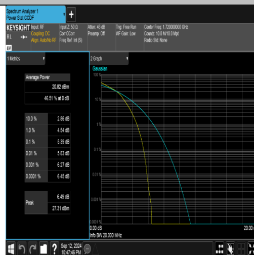
Band4-20MHz-16QAM-20050-100RB#0-PASS
