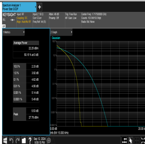
Band4-15MHz-QPSK-20025-75RB#0-PASS
