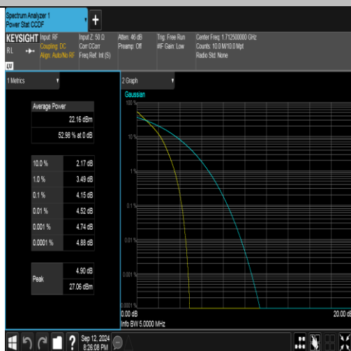
Band4-5MHz-QPSK-19975-25RB#0-PASS
