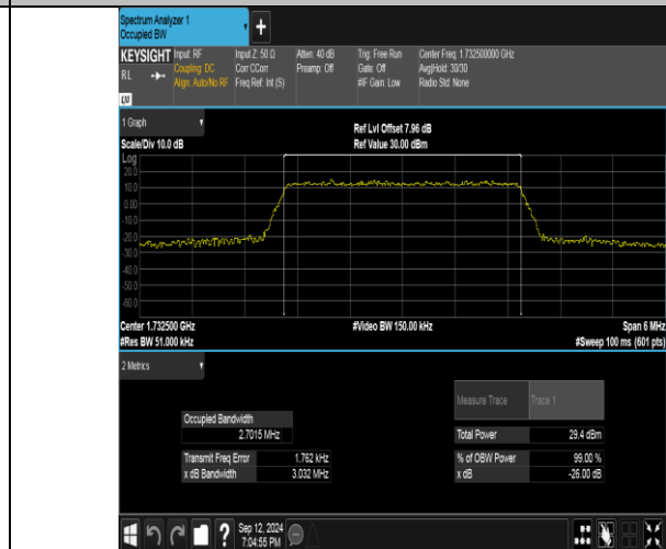
Band4-3MHz-16QAM-20175-15RB#0-PASS
