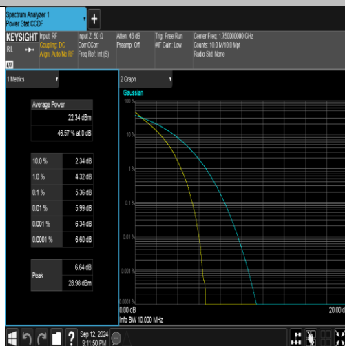
Band4-10MHz-QPSK-20350-50RB#0-PASS
