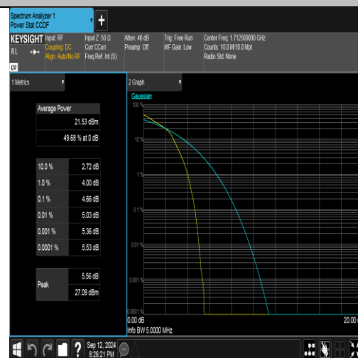
Band4-5MHz-16QAM-19975-25RB#0-PASS
