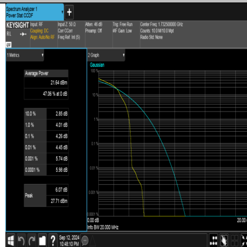
Band4-20MHz-16QAM-20175-1RB#0-PASS
