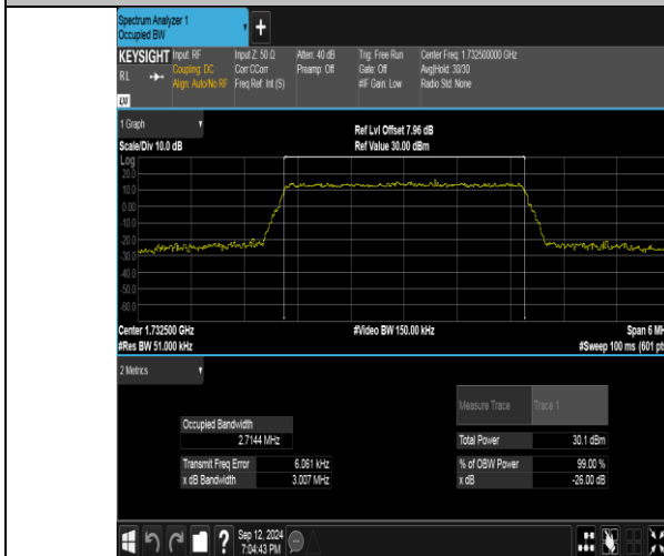
Band4-3MHz-QPSK-20175-15RB#0-PASS
