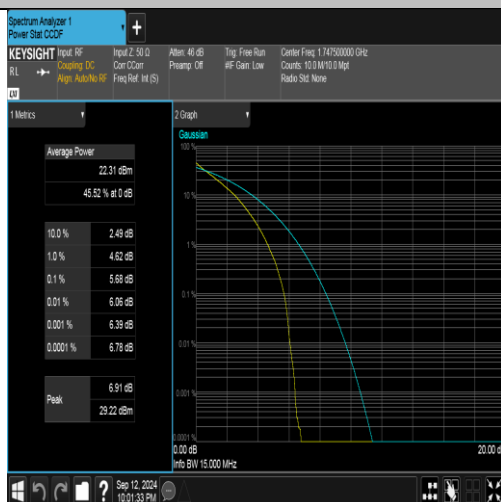
Band4-15MHz-QPSK-20325-75RB#0-PASS
