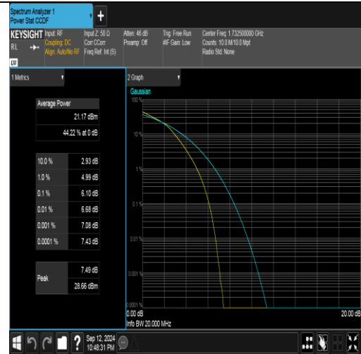
Band4-20MHz-16QAM-20175-100RB#0-PASS
