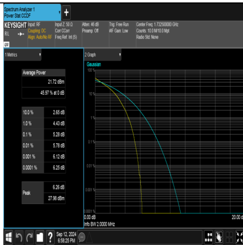
Band4-1.4MHz-QPSK-20175-6RB#0-PASS
