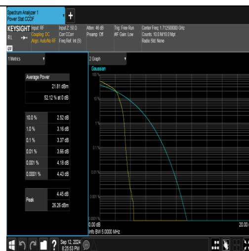
Band4-5MHz-16QAM-19975-1RB#0-PASS
