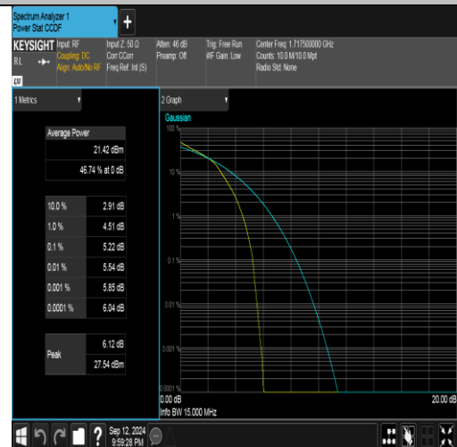
Band4-15MHz-16QAM-20025-75RB#0-PASS
