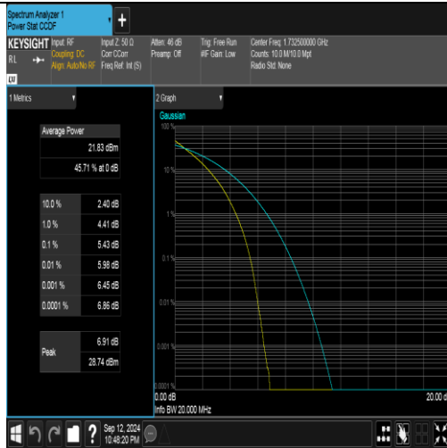
Band4-20MHz-QPSK-20175-100RB#0-PASS
