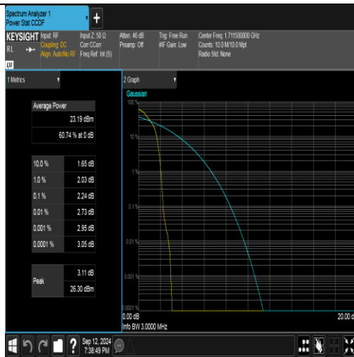
Band4-3MHz-QPSK-19965-1RB#0-PASS
