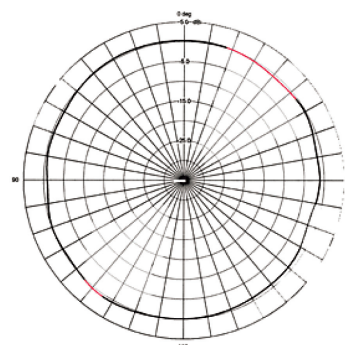
TYPICAL AZIMUTH GAIN
