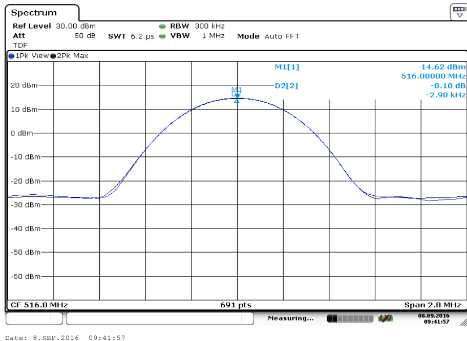
Plot 3: highest channel, conducted peak power
