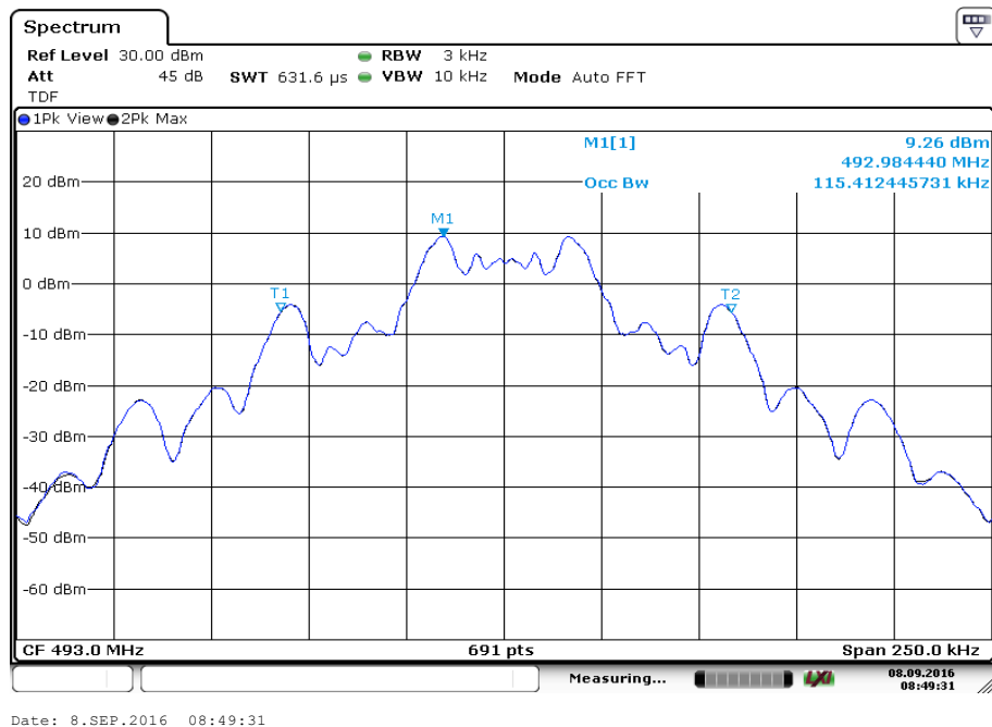
Plot 2: middle channel, 2.5 kHz tone
