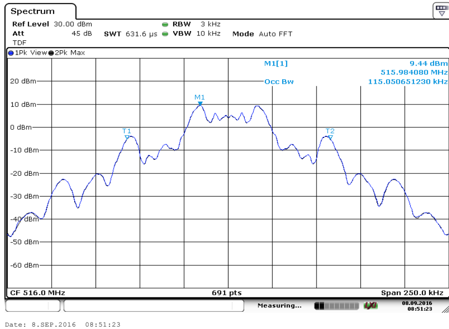
Plot 3: highest channel, 2.5 kHz tone
