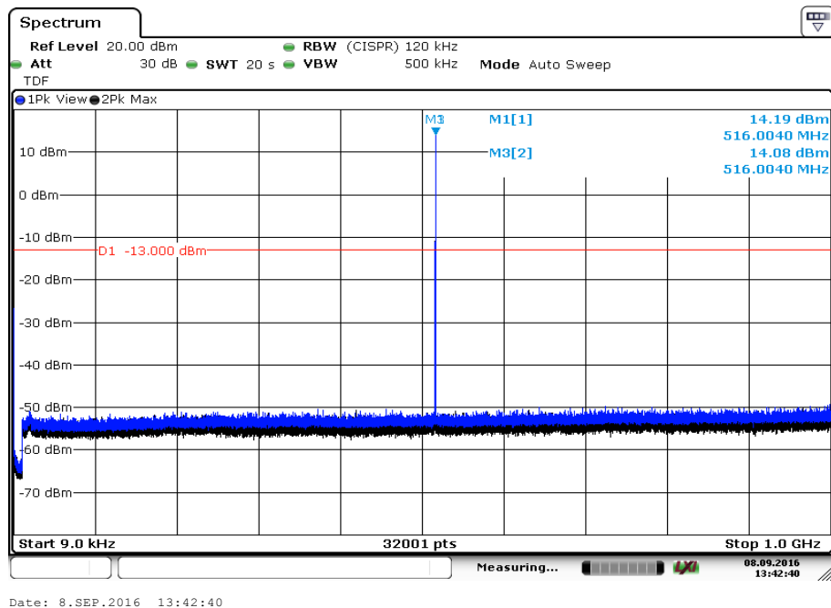
Plot 5: highest channel, 9 kHz to 1 GHz, FCC requirement
