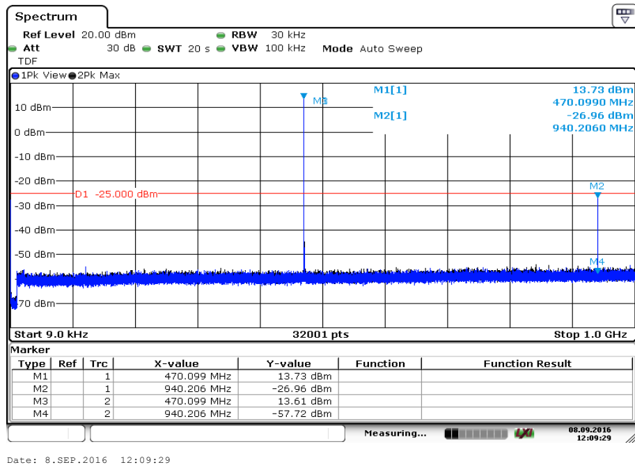
Plot 7: lowest channel, 9 kHz to 1 GHz, IC requirement
