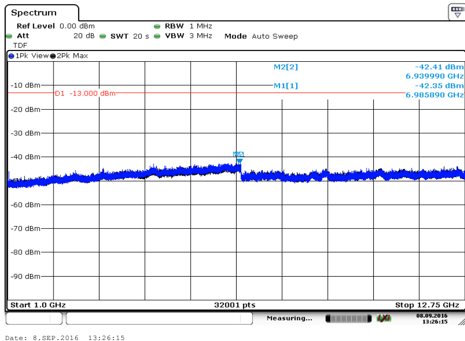
Plot 6: highest channel, 1 GHz to 12.75 GHz, FCC requirement
