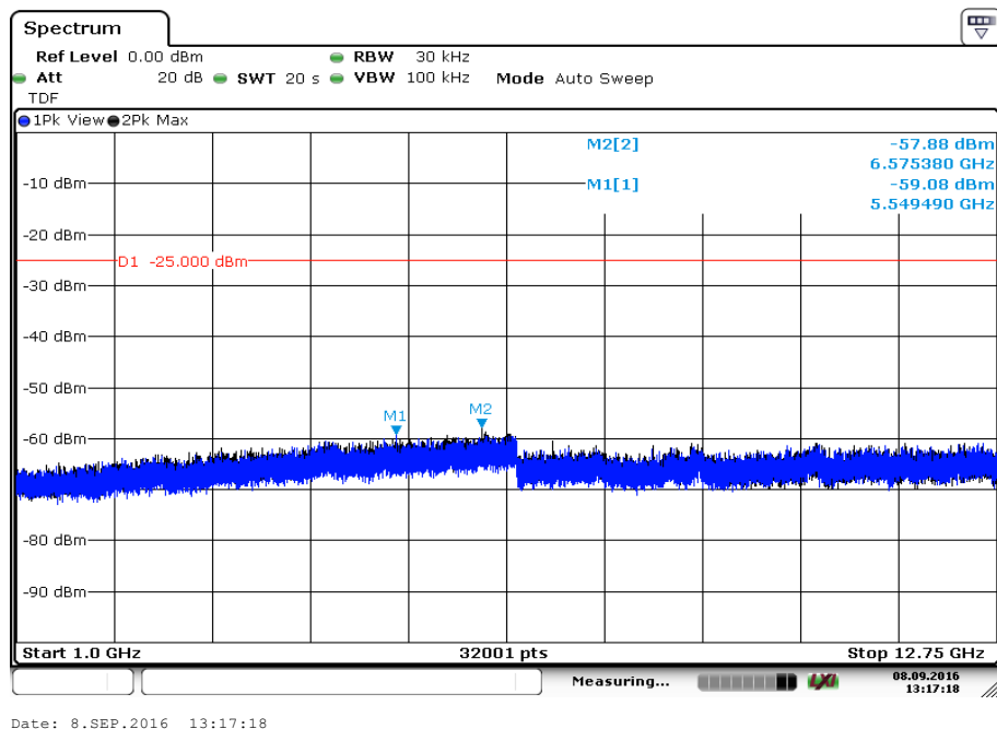
Plot 8: lowest channel, 1 GHz to 12.75 GHz, IC requirement
