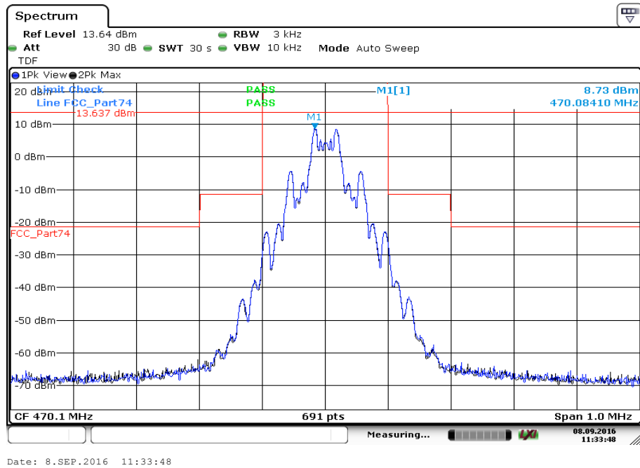
Plot 3: lowest channel, spectrum mask
