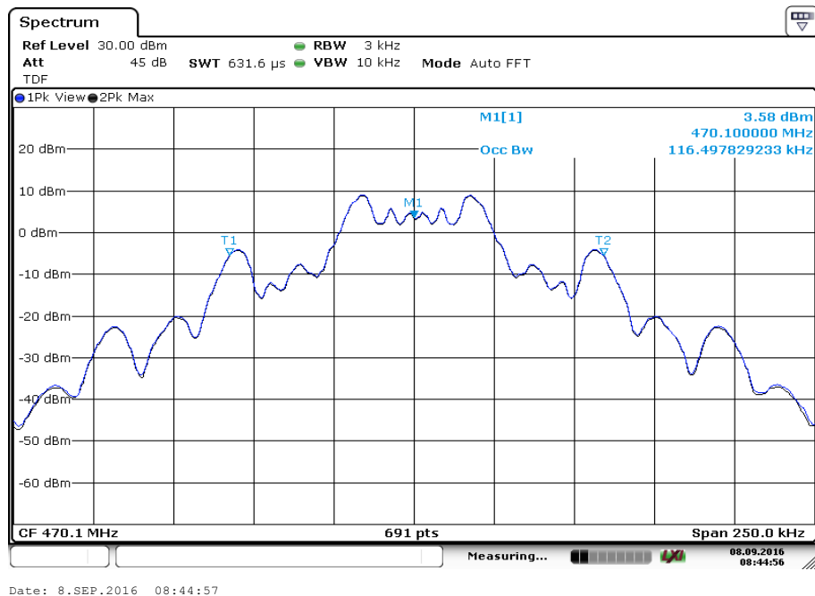
Plot 1: lowest channel, 2.5 kHz tone
