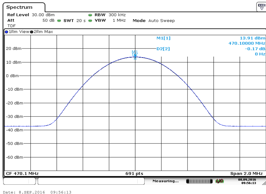
Plot 4: lowest channel, conducted average power
